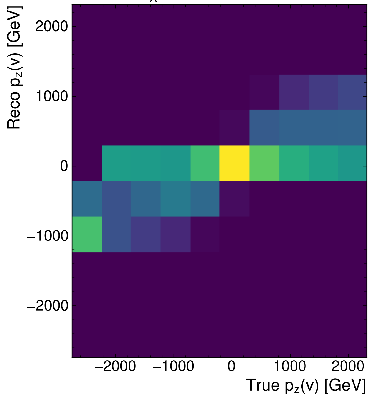
\chi^2 -Method v^2 -Flows
