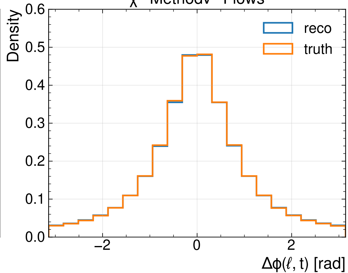
\chi^2 -Method v^2 -Flows
