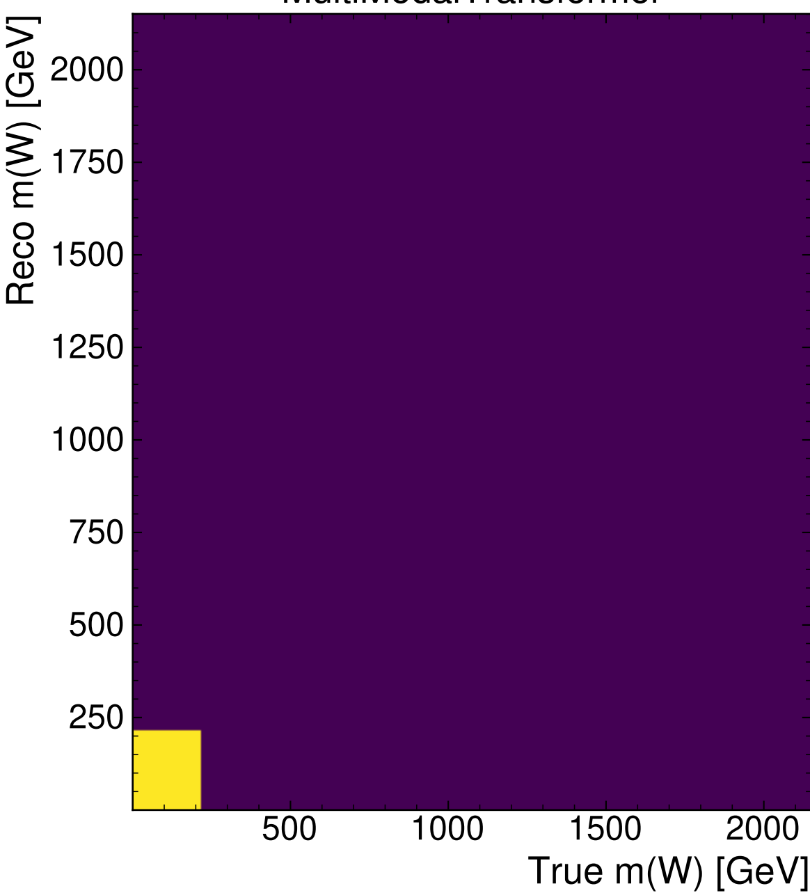
MultiModalTransformer
