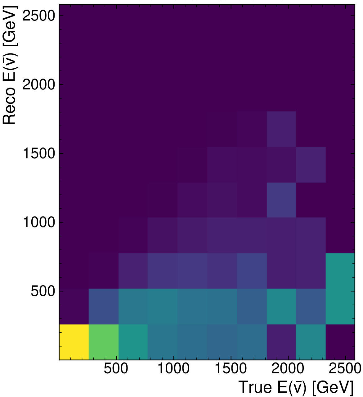
MultiModalTransformer
