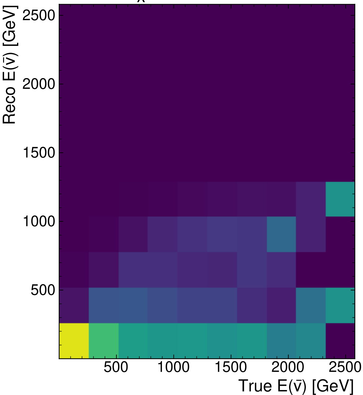
MultiModalTransformer
