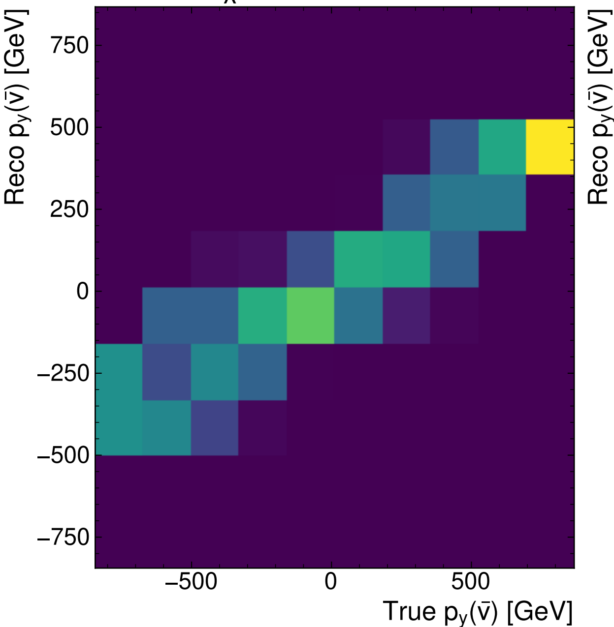
MultiModalTransformer
