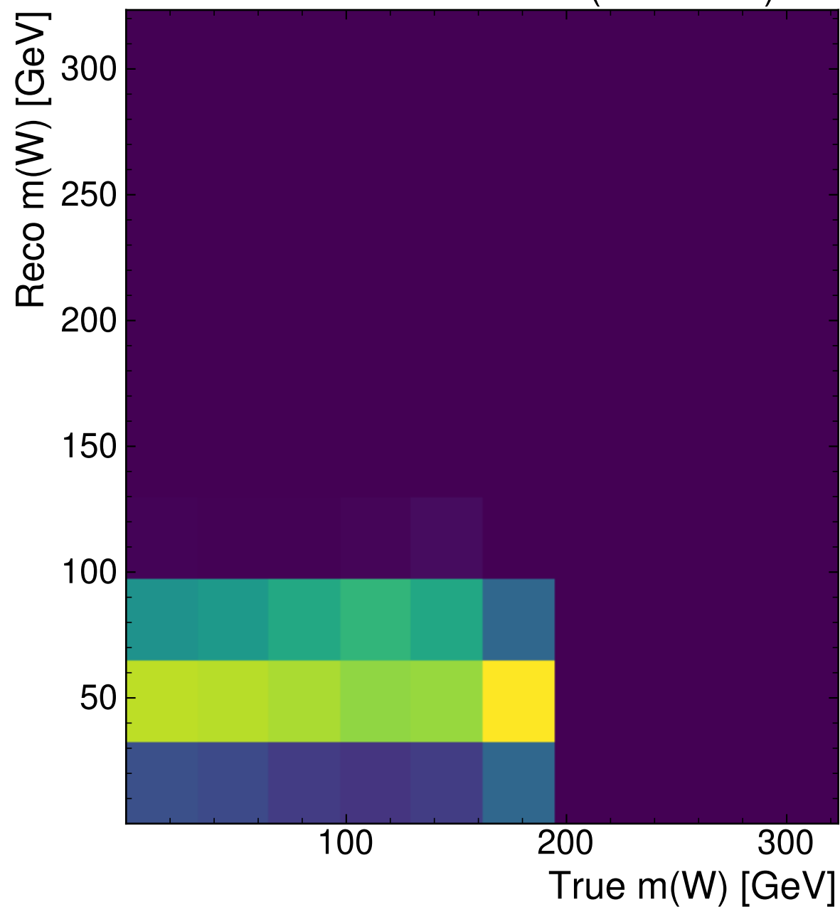
MultiModelTransformer (Magnitude-Direction)
