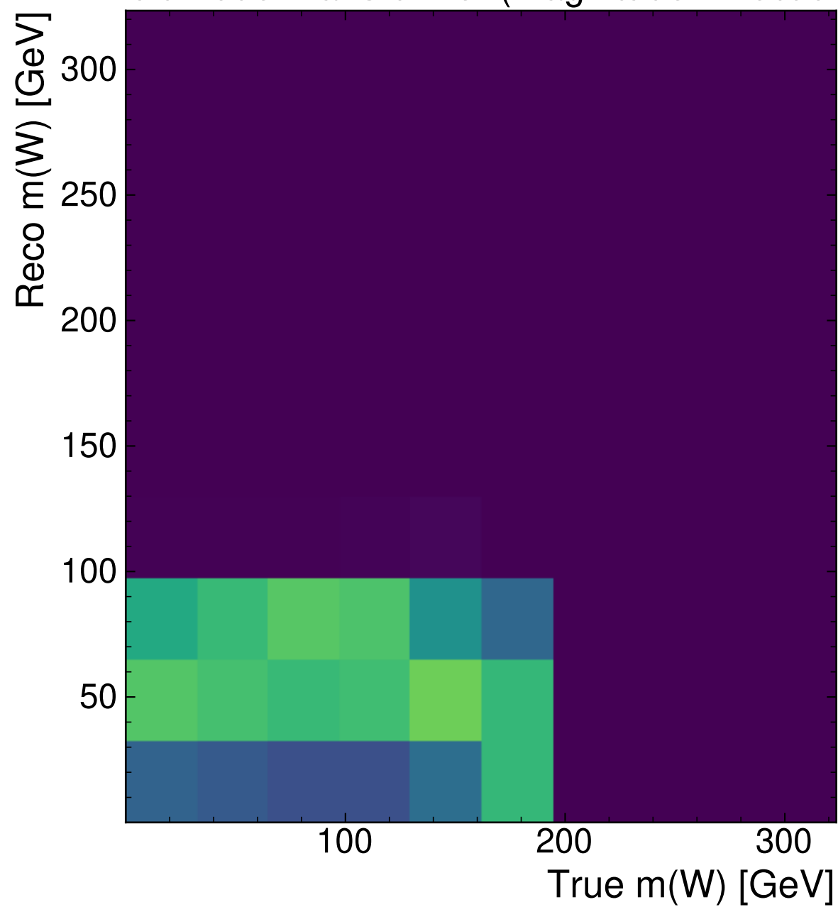
MultiModelTransformer (Magnitude-Direction)
