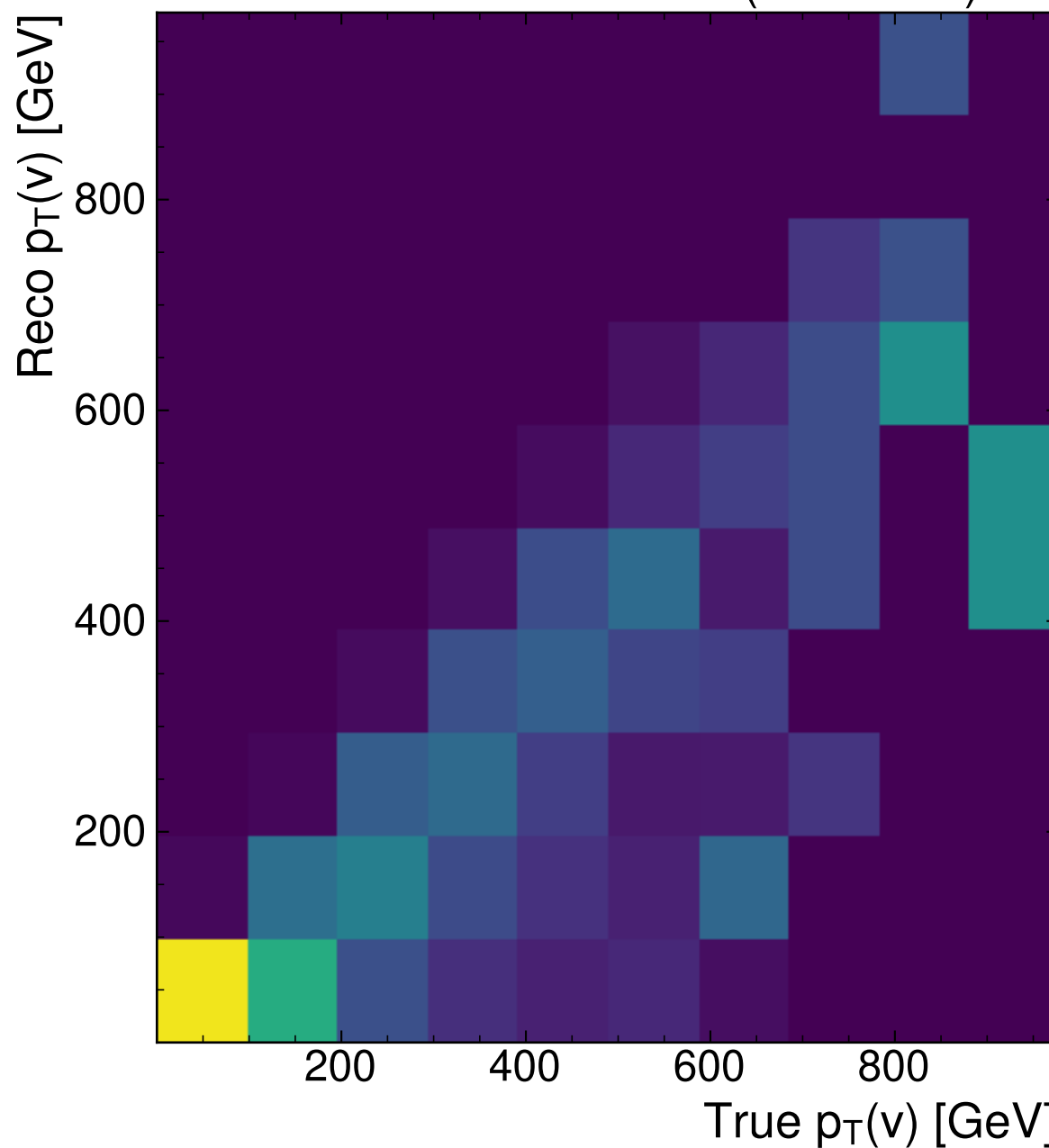
MultiModelTransformer (Magnitude-Direction)
