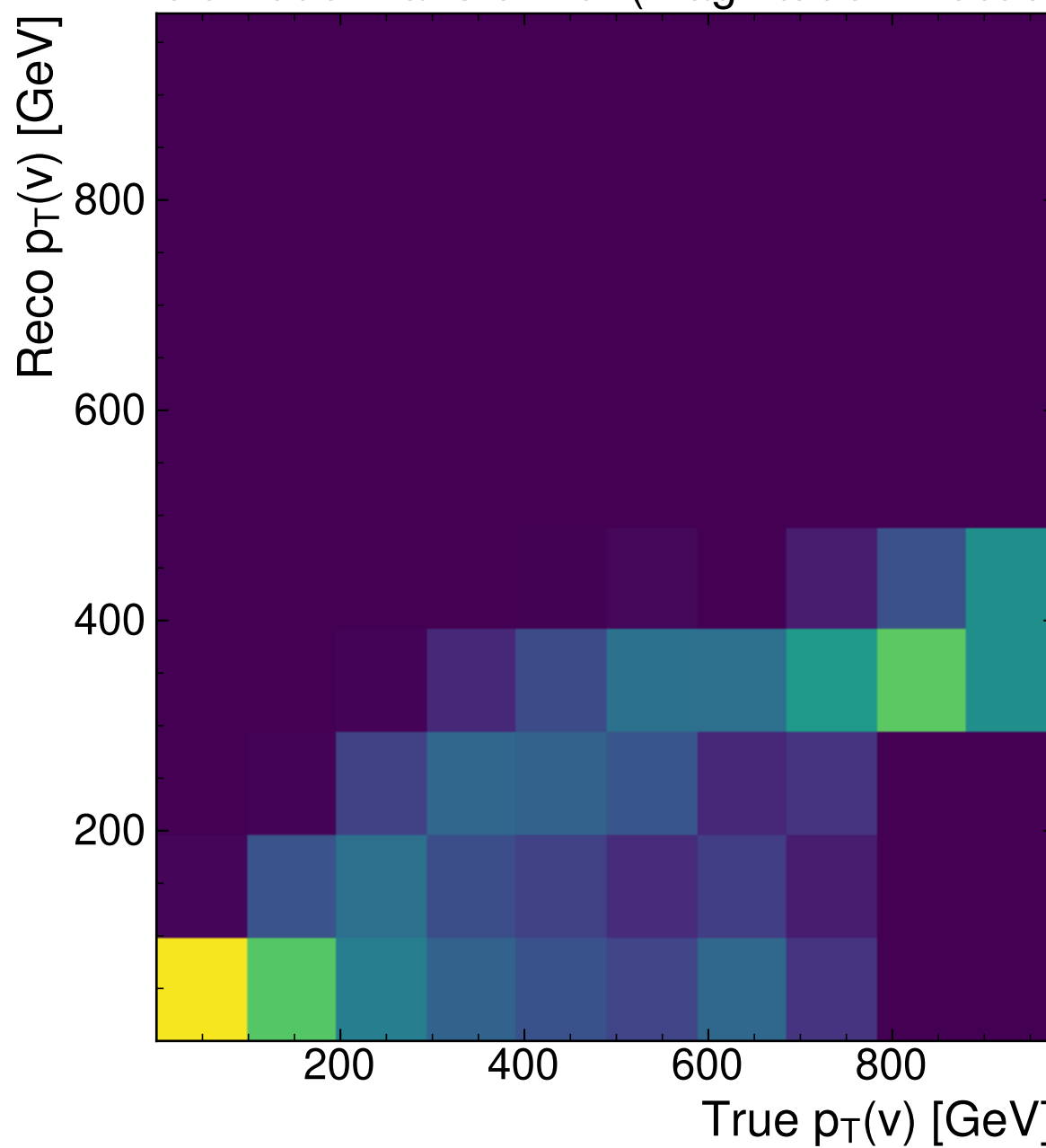
MultiModelTransformer (Magnitude-Direction)
