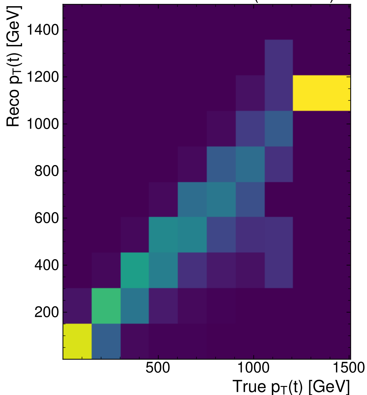
MultiModelTransformer (Magnitude-Direction)
