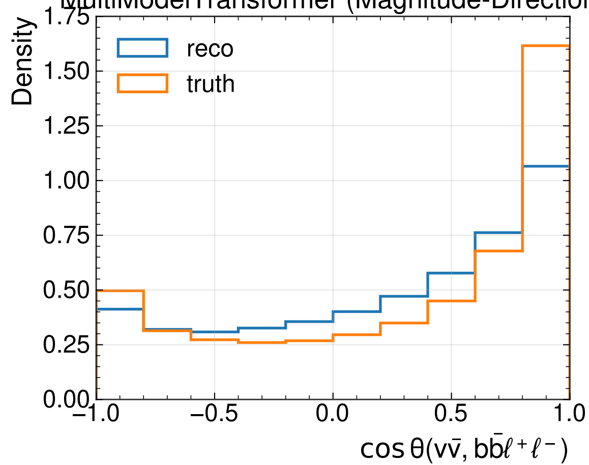
MultiModelTransformer (Magnitude-Direction)
