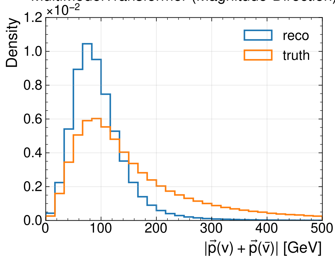
MultiModelTransformer (Magnitude-Direction)
