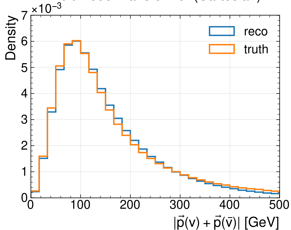
MultiModelTransformer (Magnitude-Direction)
