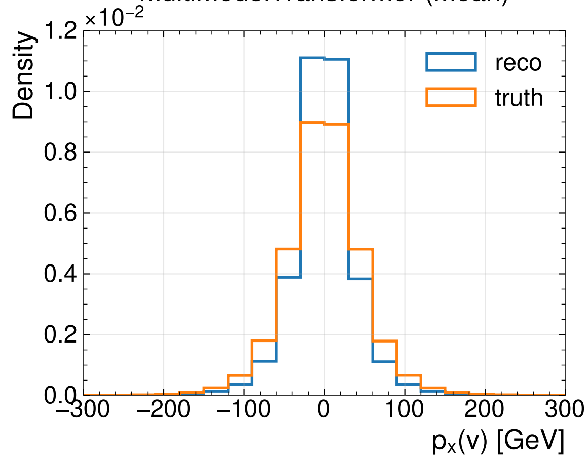
MultiModelTransformer (Mean)
