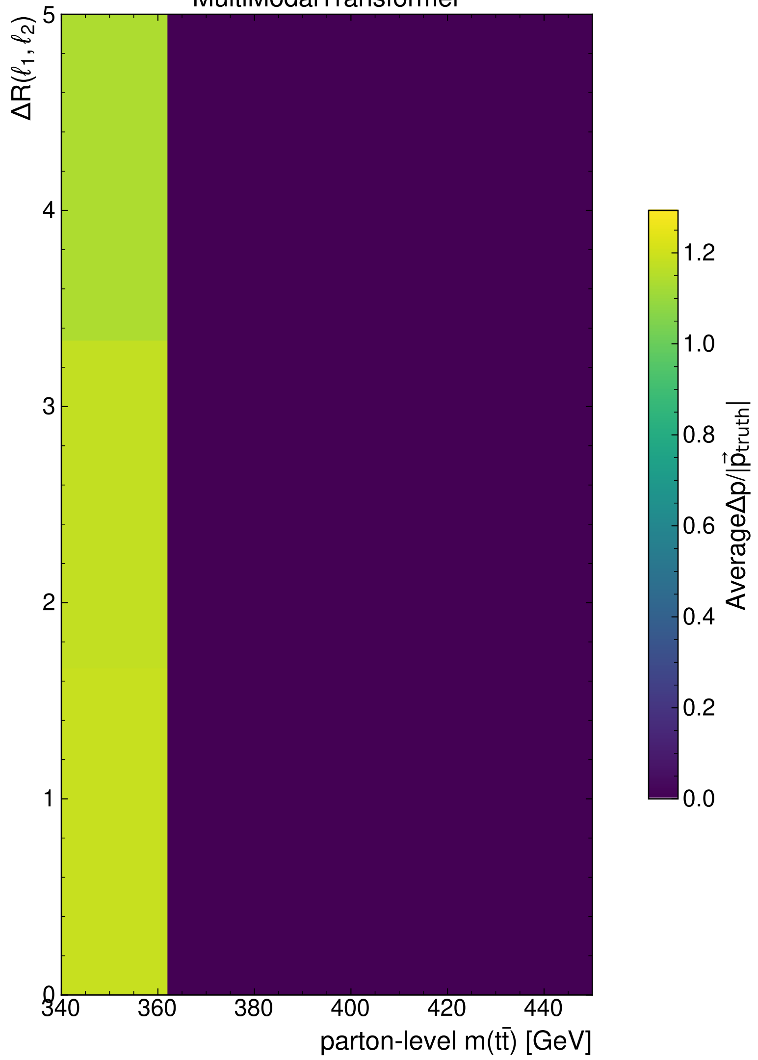
MultiModalTransformer
