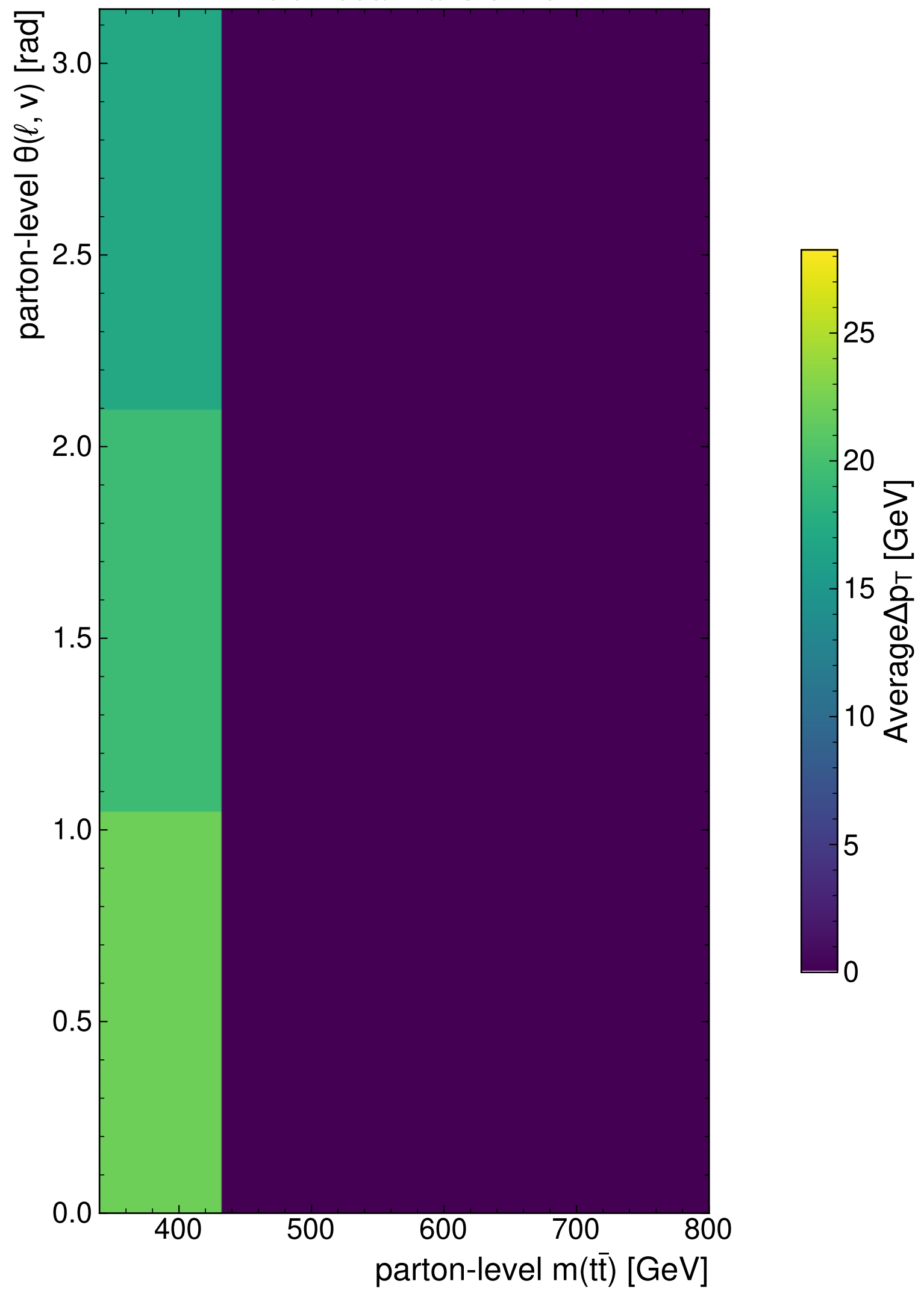
MultiModalTransformer
