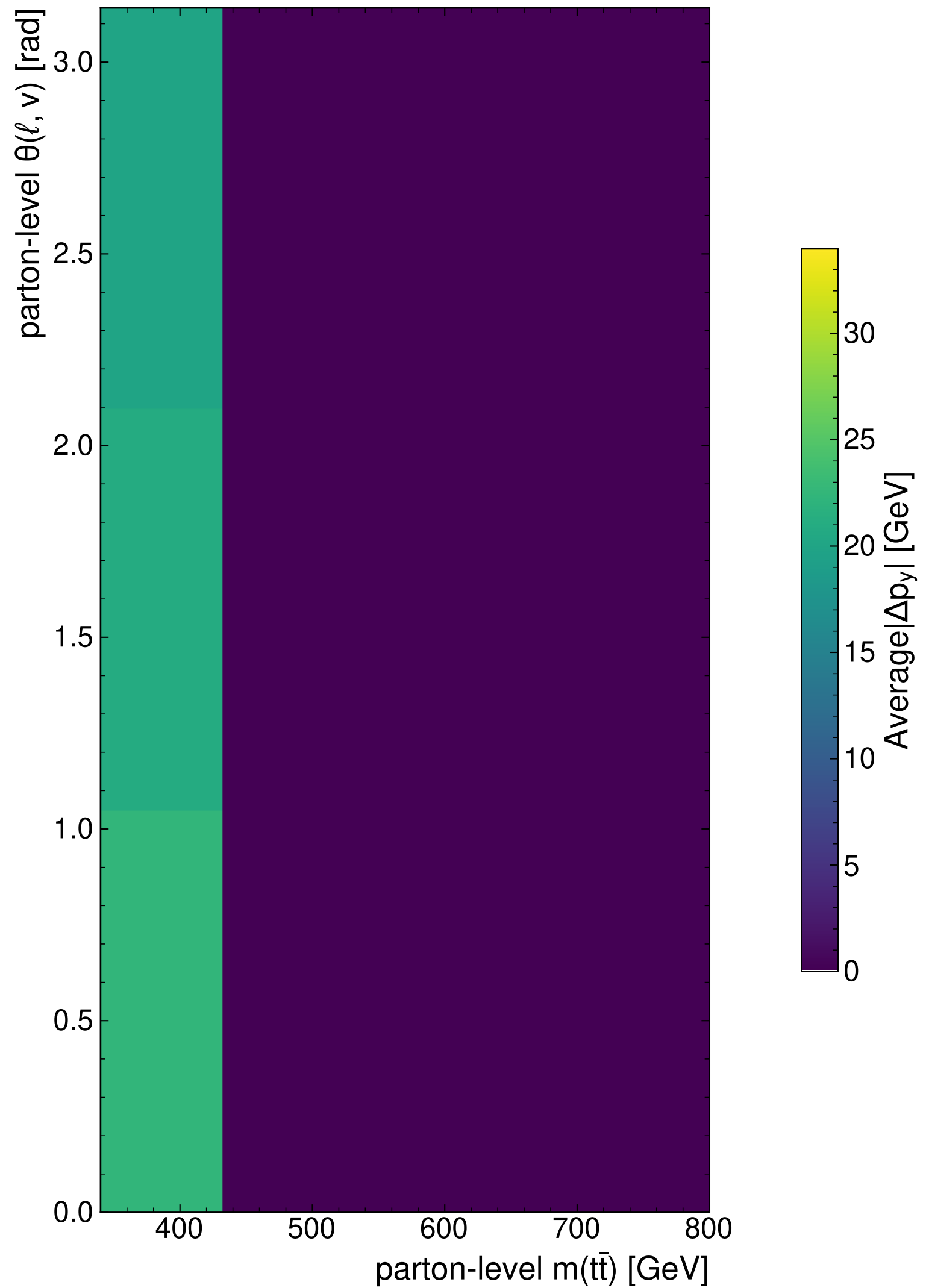
MultiModalTransformer
