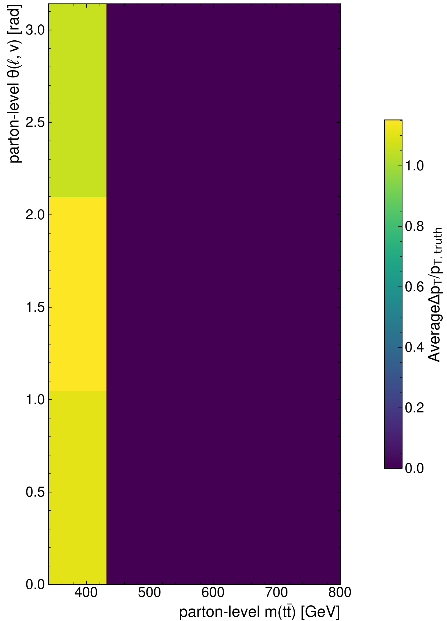
MultiModalTransformer
