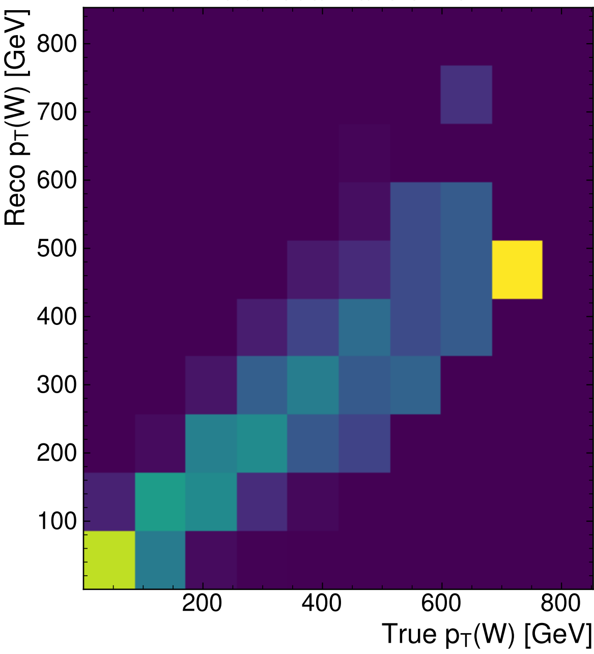
MultiModalTransformer
