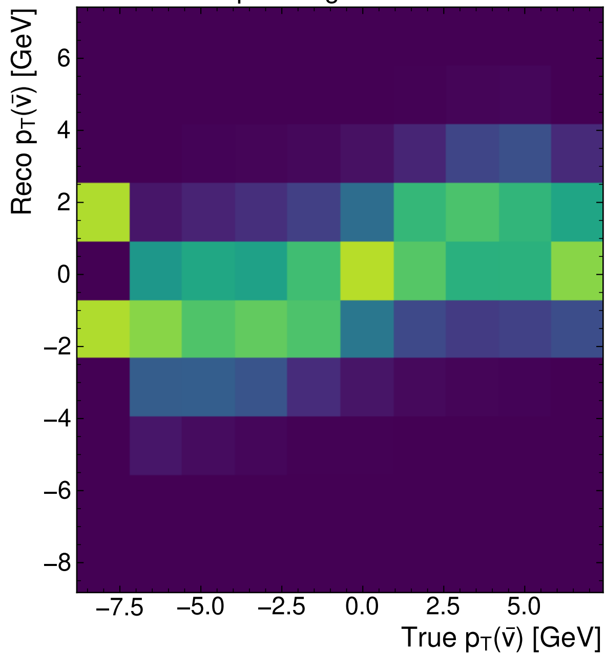
ComapctAssigner + v^2 -Flows
