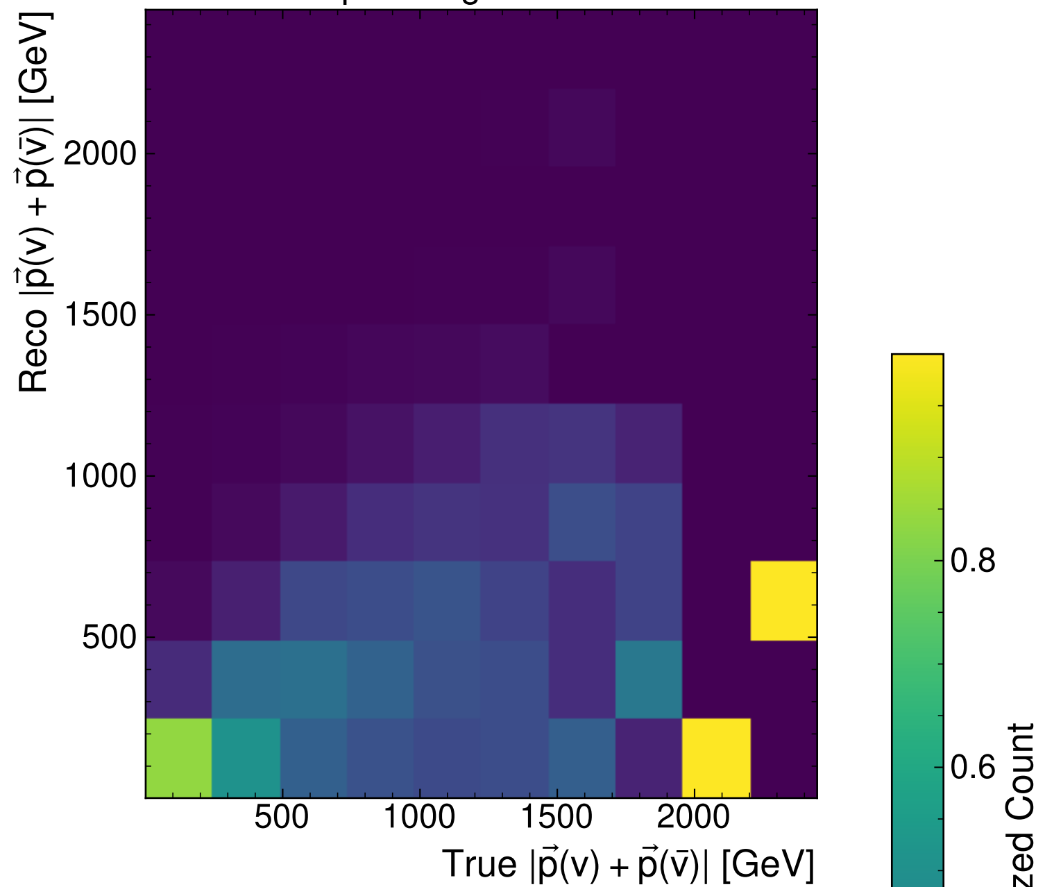
ComapctAssigner + v^2 -Flows
