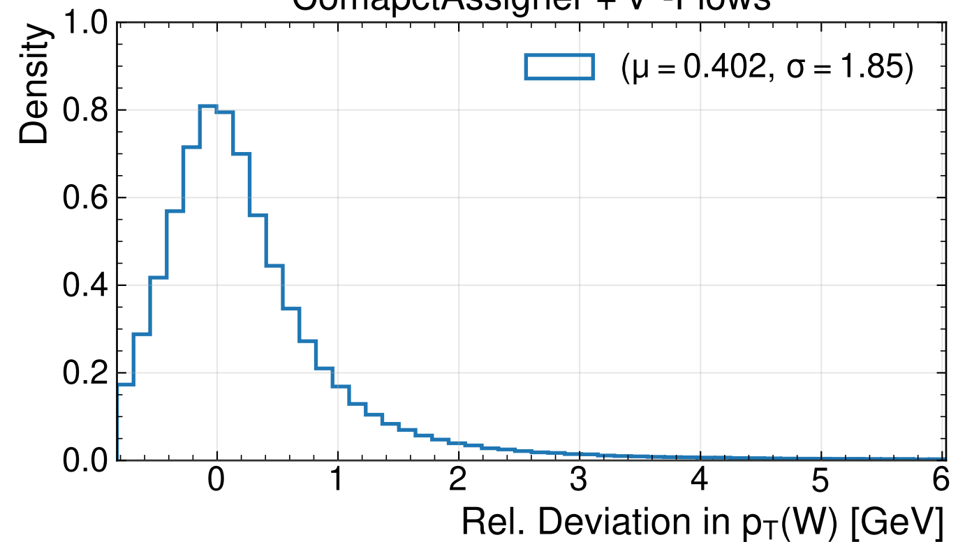
ComapctAssigner + v^2 -Flows
