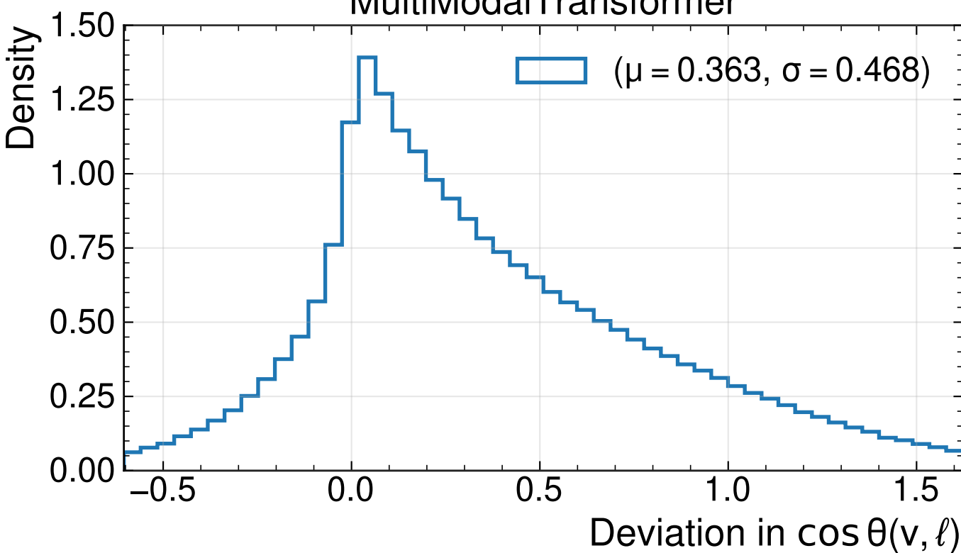
MultiModalTransformer
