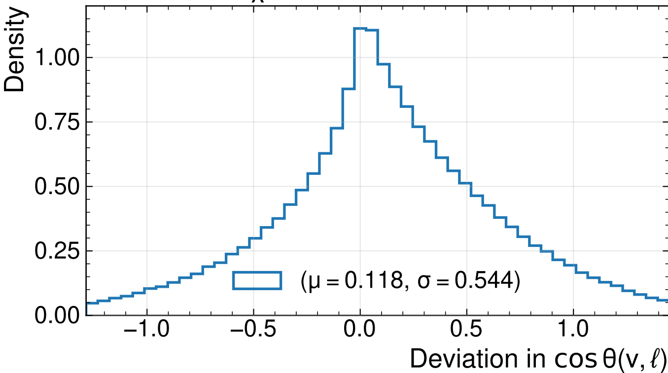
MultiModalTransformer
