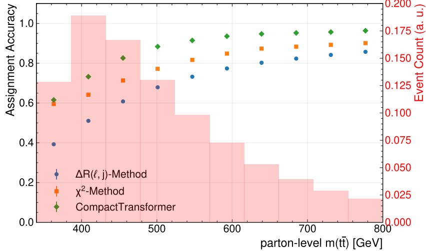
Figure 7.2.: This plot shows the assignment accuracy in bins of the true invariant mass of the top-quark pair.
