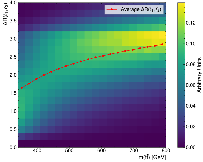
Figure A.5.: This plot shows the distribution of events binned in the parton-level m(t\bar{t}) and the angular distance \Delta R(\ell_1, \ell_2) .
