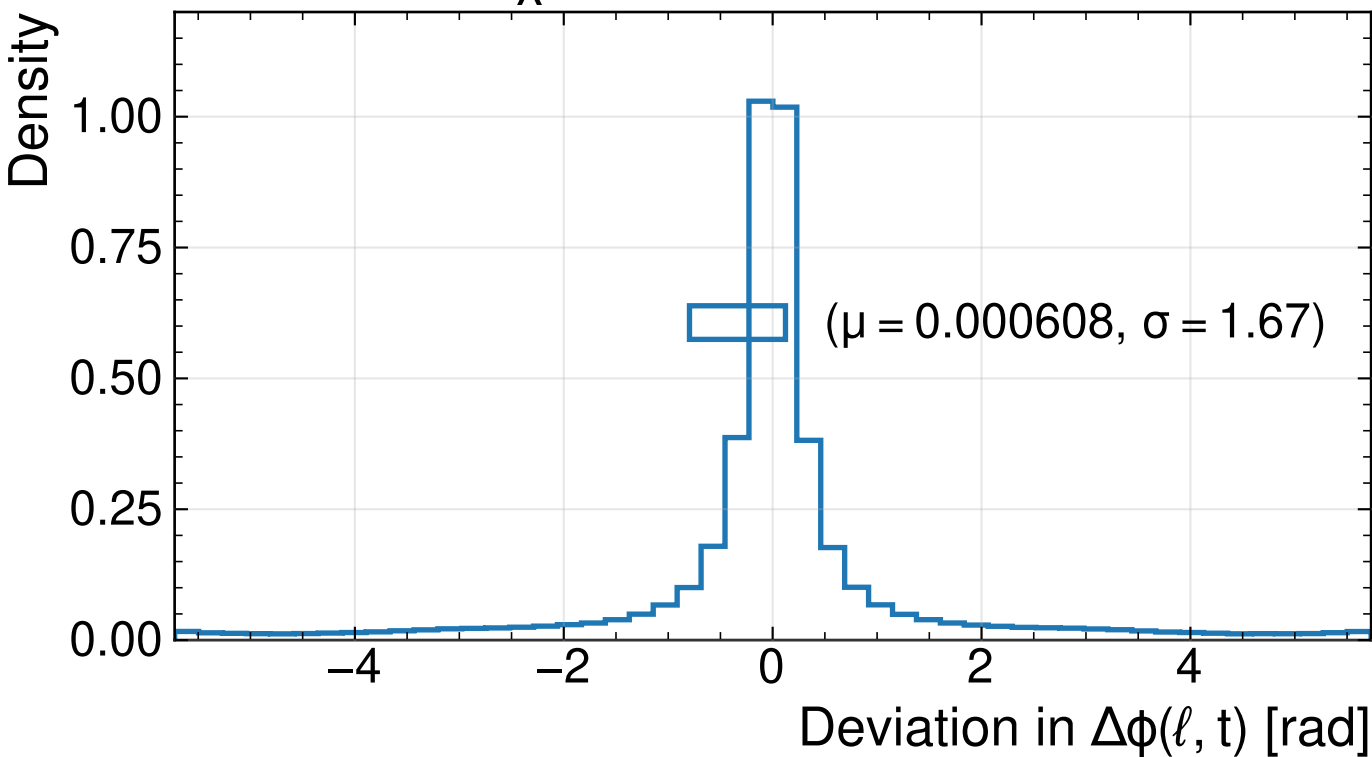
MultiModalTransformer
