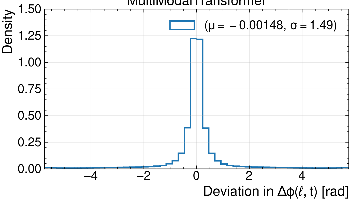
MultiModalTransformer
