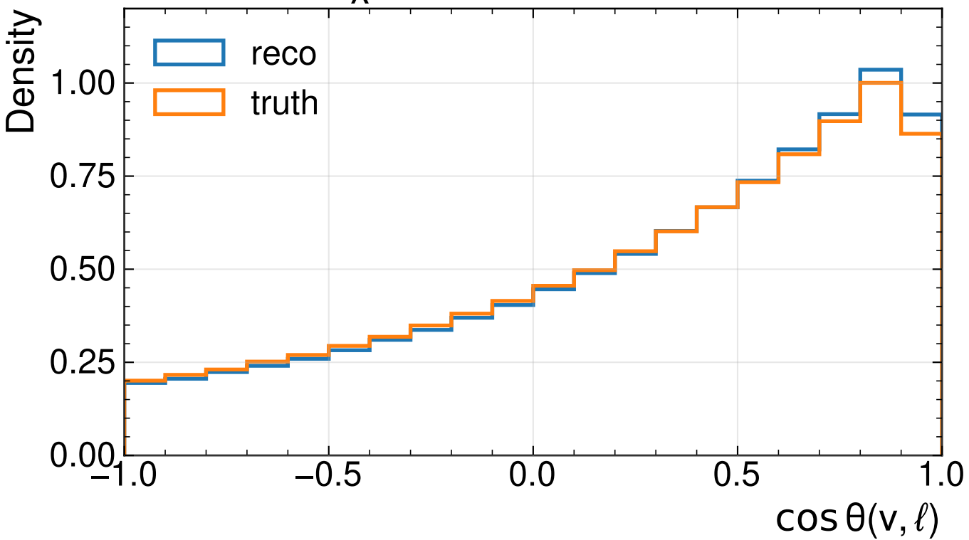
MultiModalTransformer
