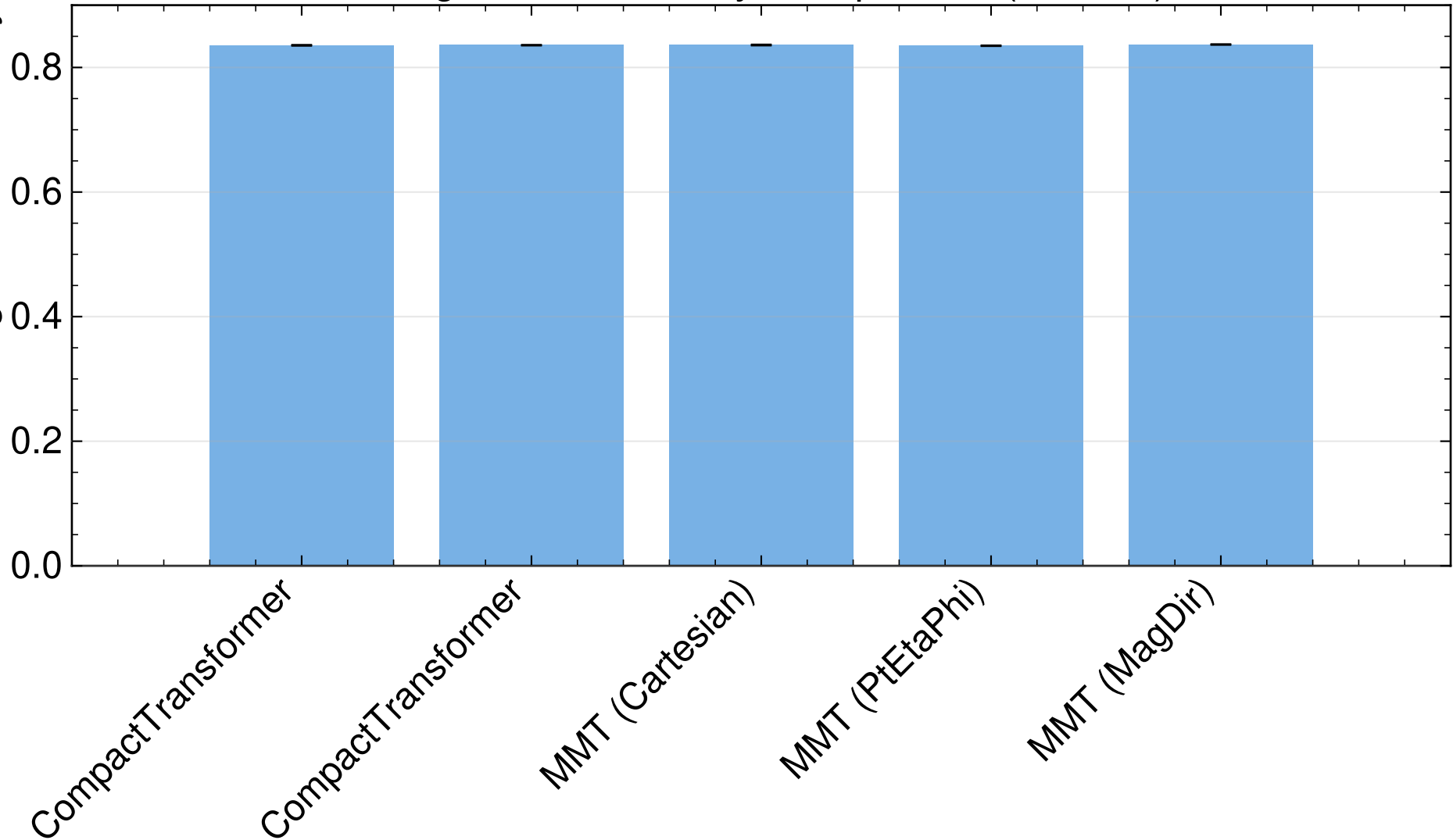
Assignment Accuracy Comparison (95% CI)
