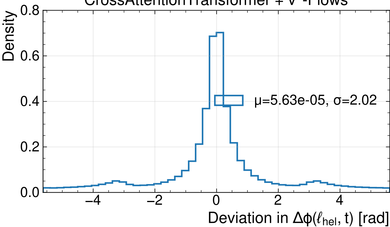
CrossAttentionTransformer + v^2 -Flows
