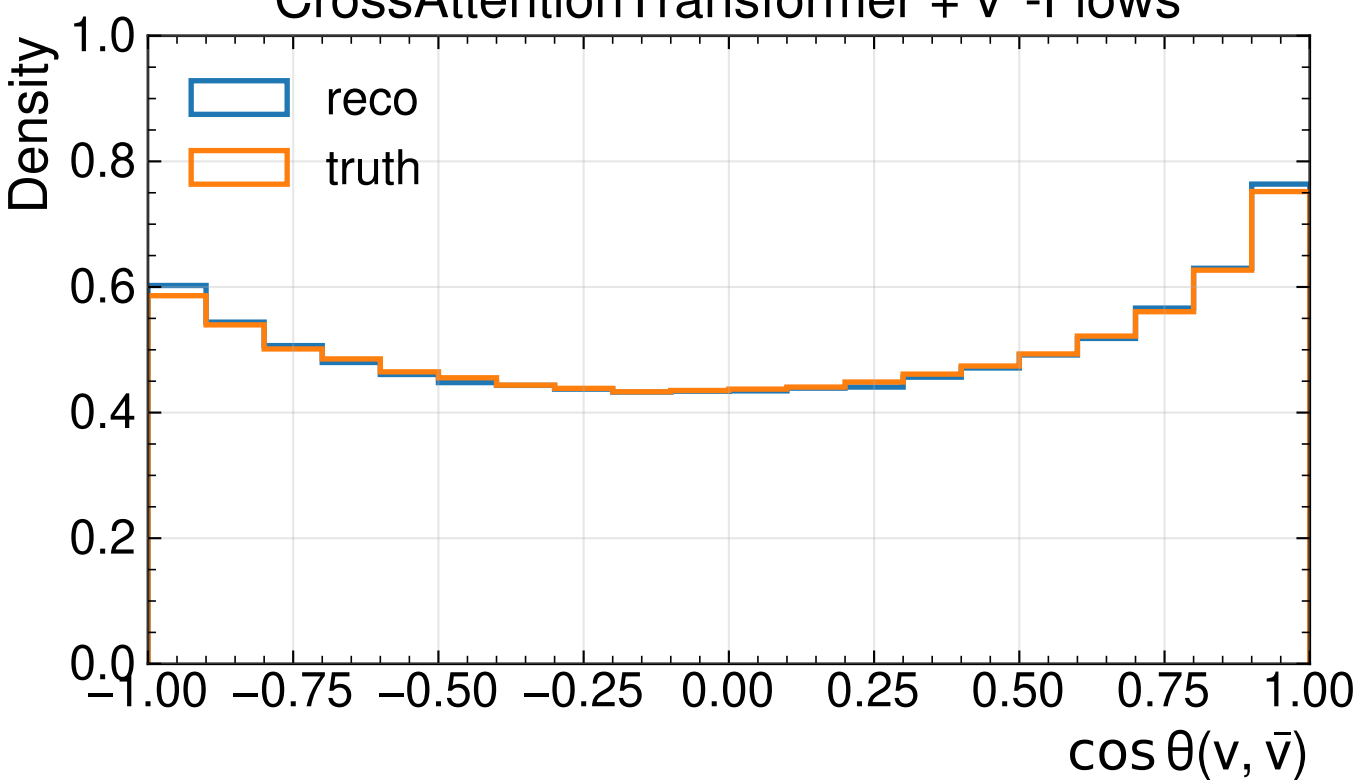
CrossAttentionTransformer + v^2 -Flows
