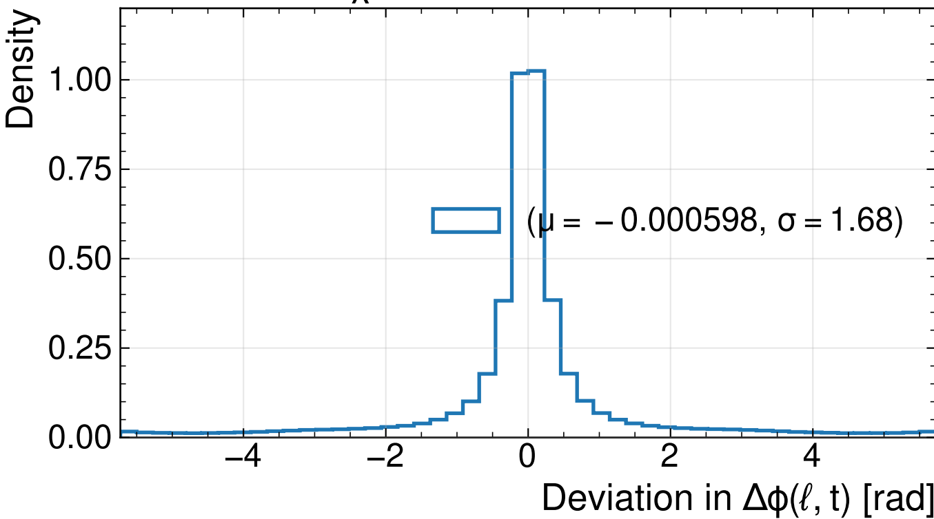
Threshold + v^2 -Flows
