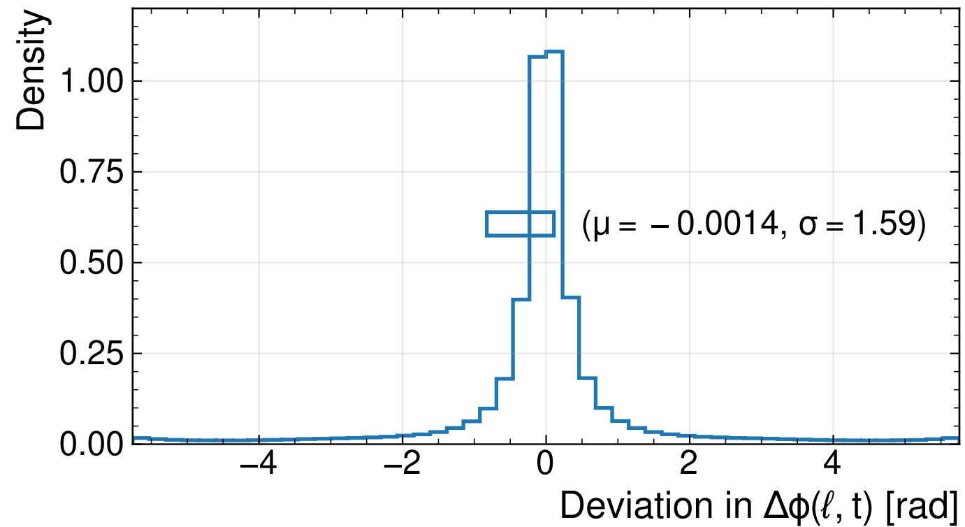
Toponium + v^2 -Flows
