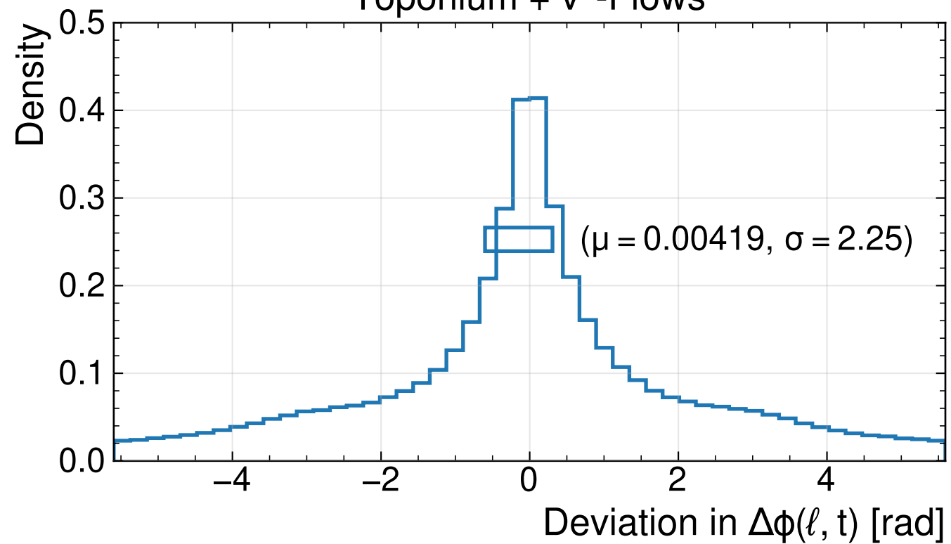
Toponium + v^2 -Flows
