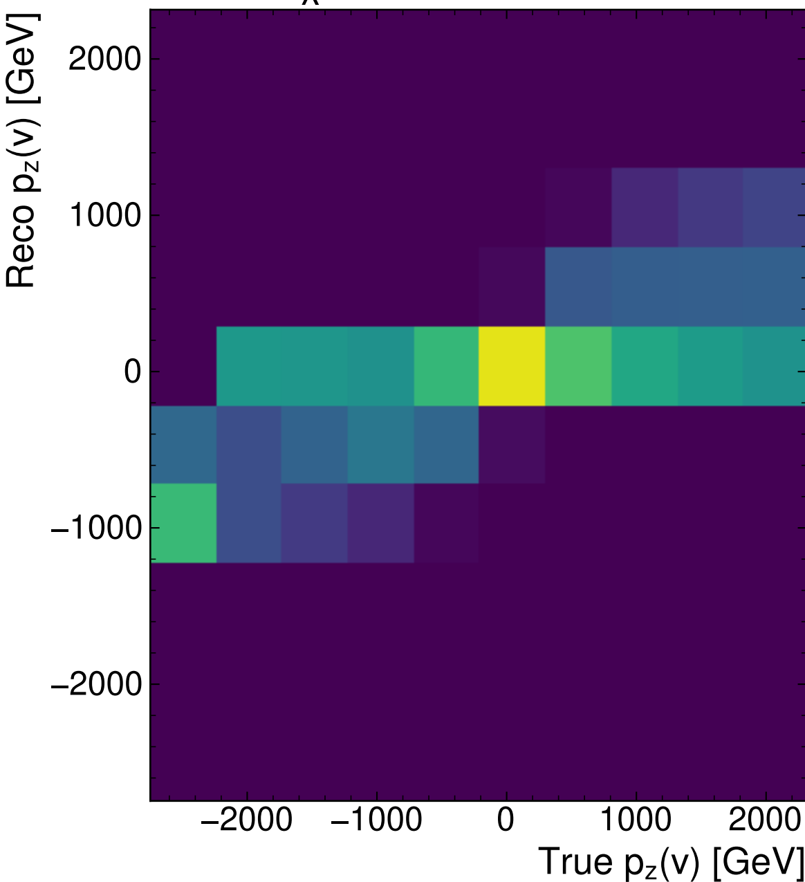
RegressionTransformer
