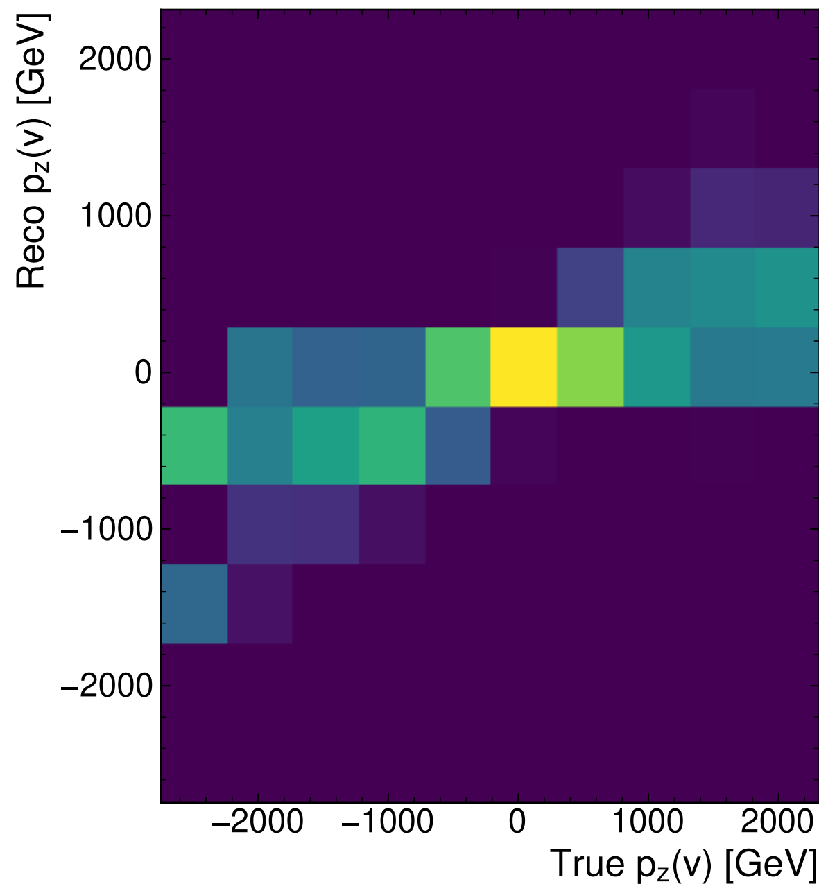
MultiModalTransformer
