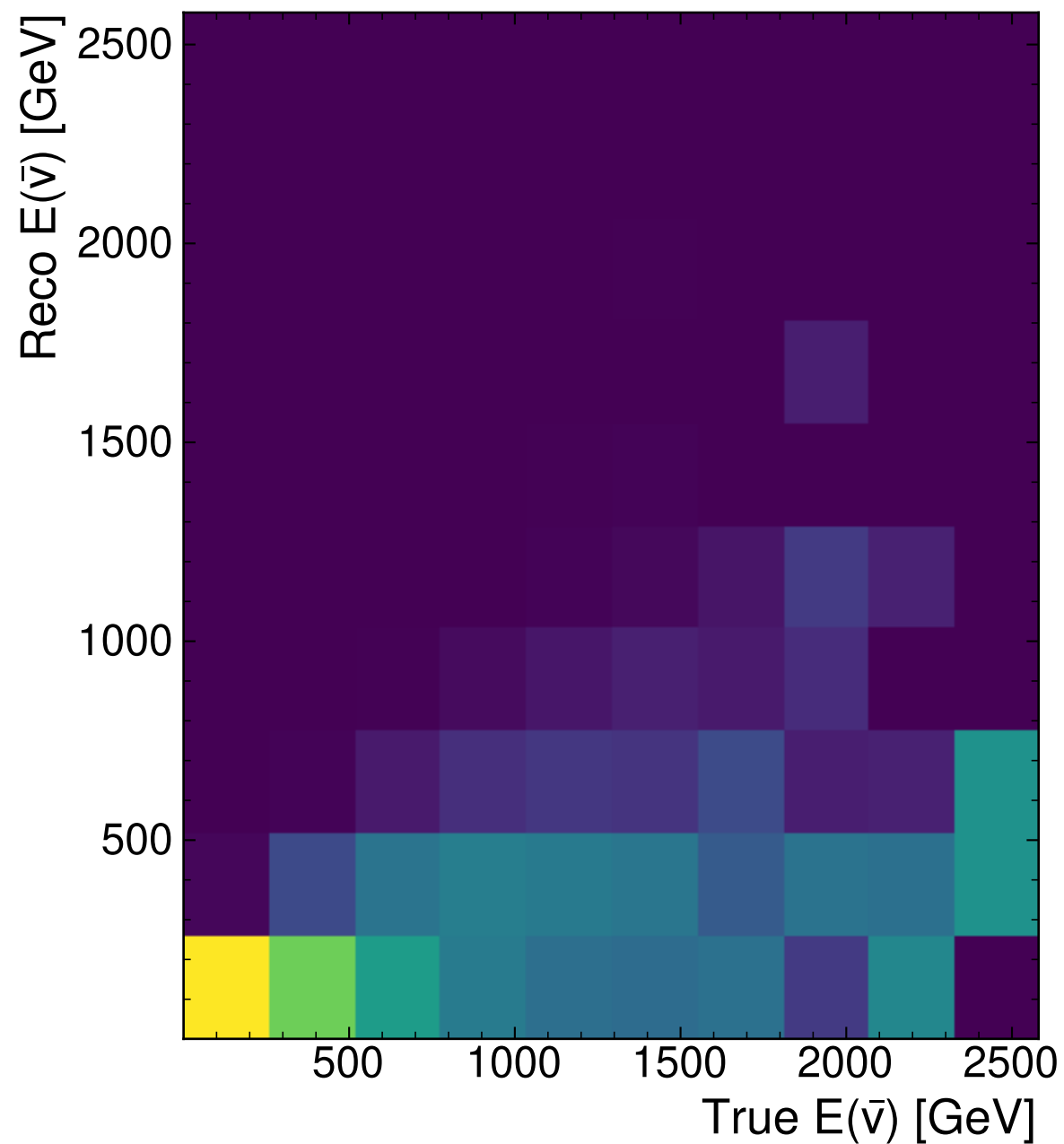
MultiModalTransformer
