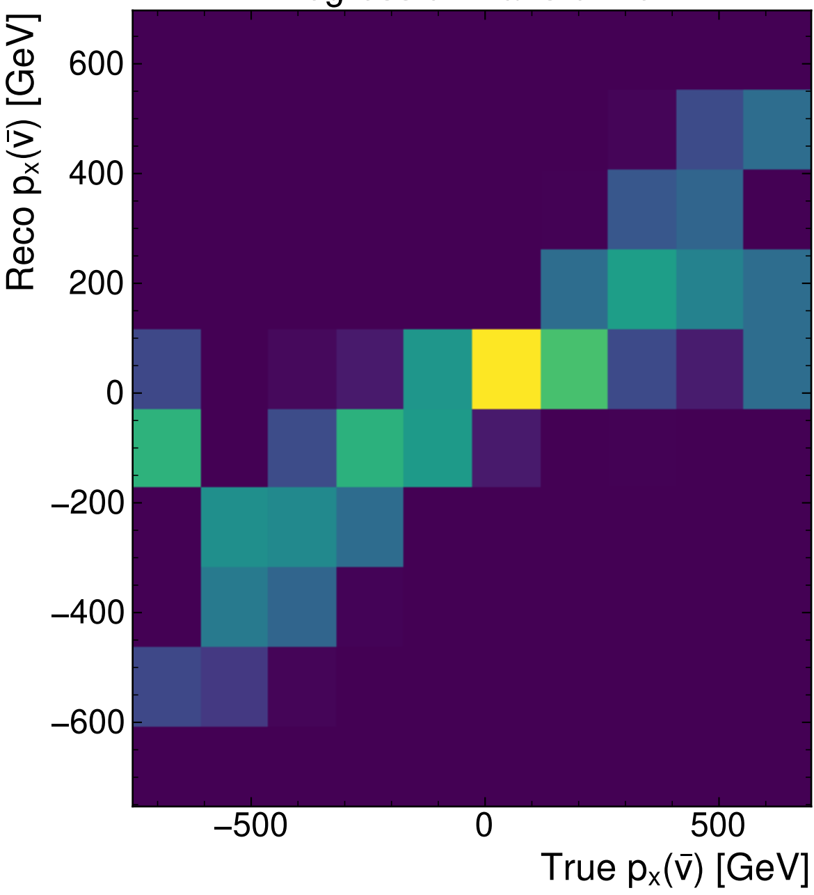
RegressionTransformer
