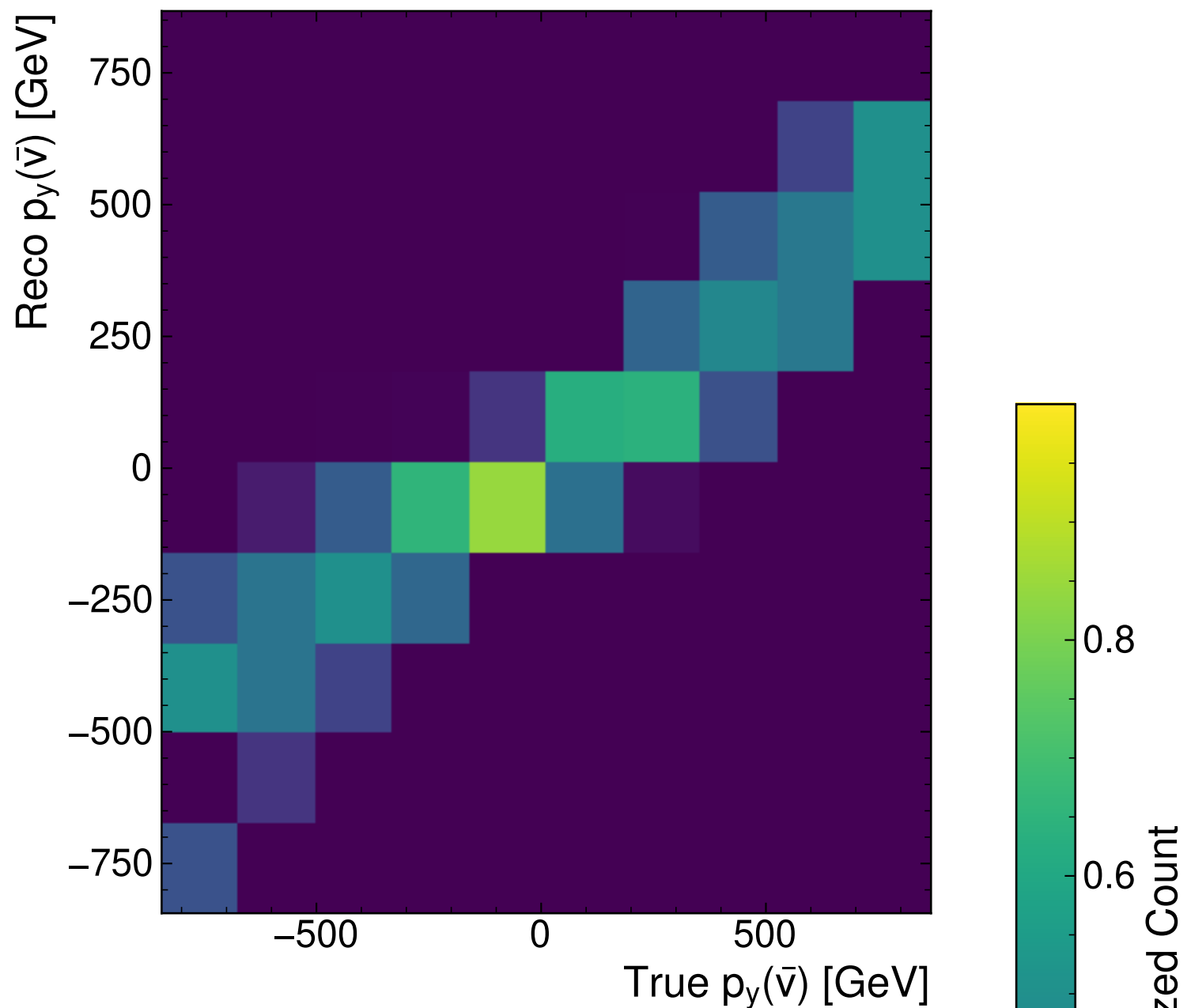
MultiModalTransformer
