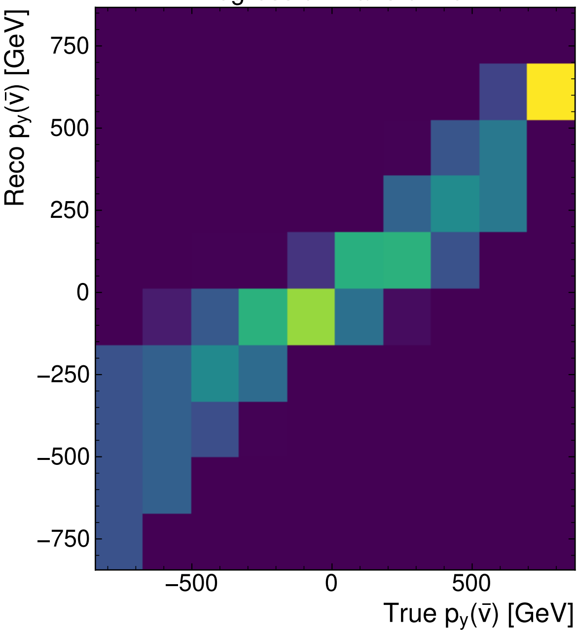
RegressionTransformer
