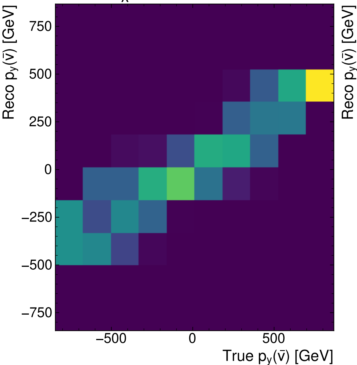
RegressionTransformer
