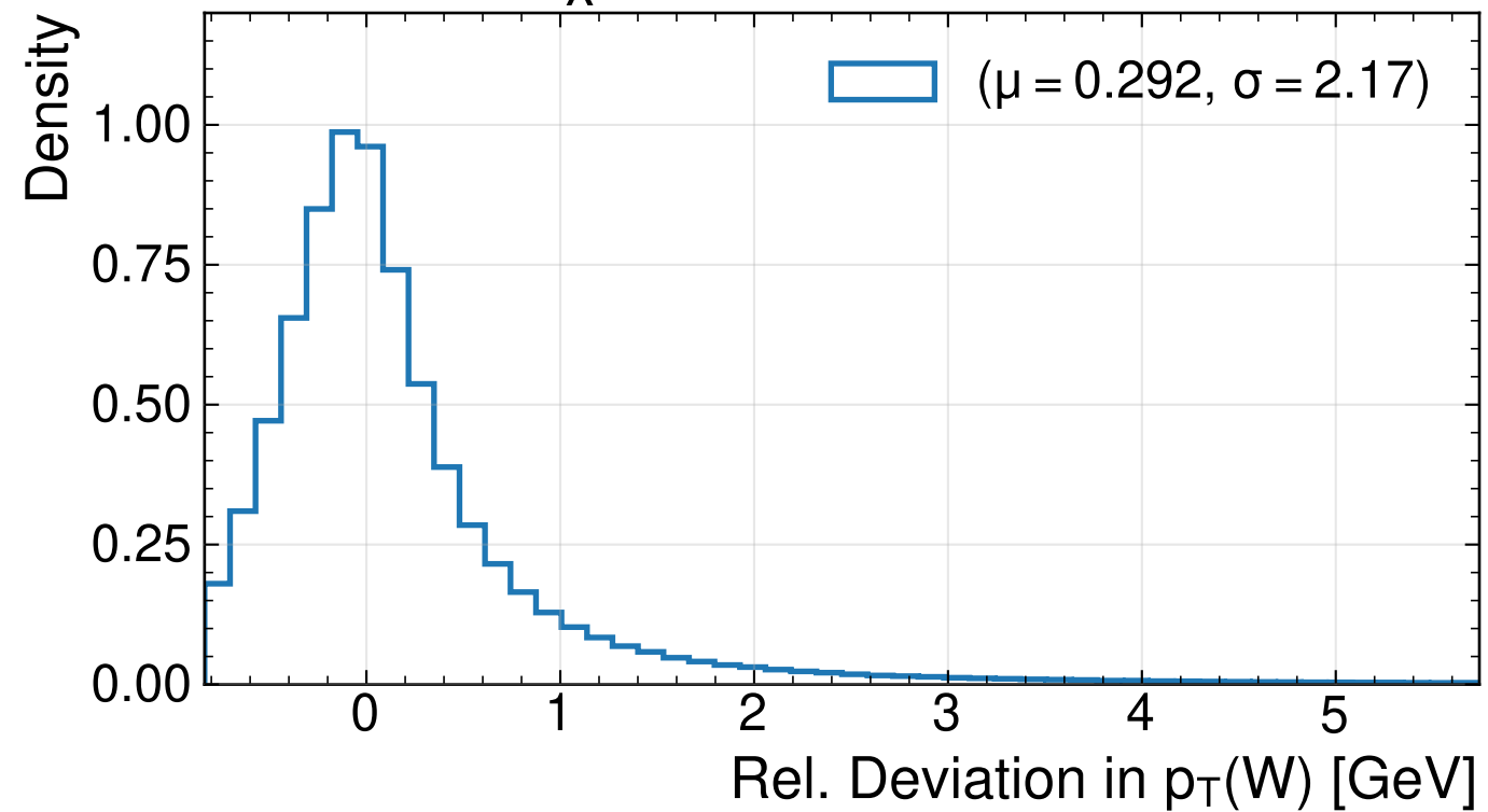
True Assignment + v^2 -Flows
