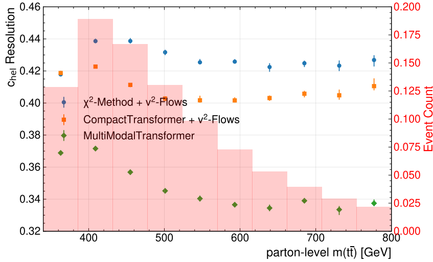
Figure 7.14.: Resolution of c_{\text{hel}}
