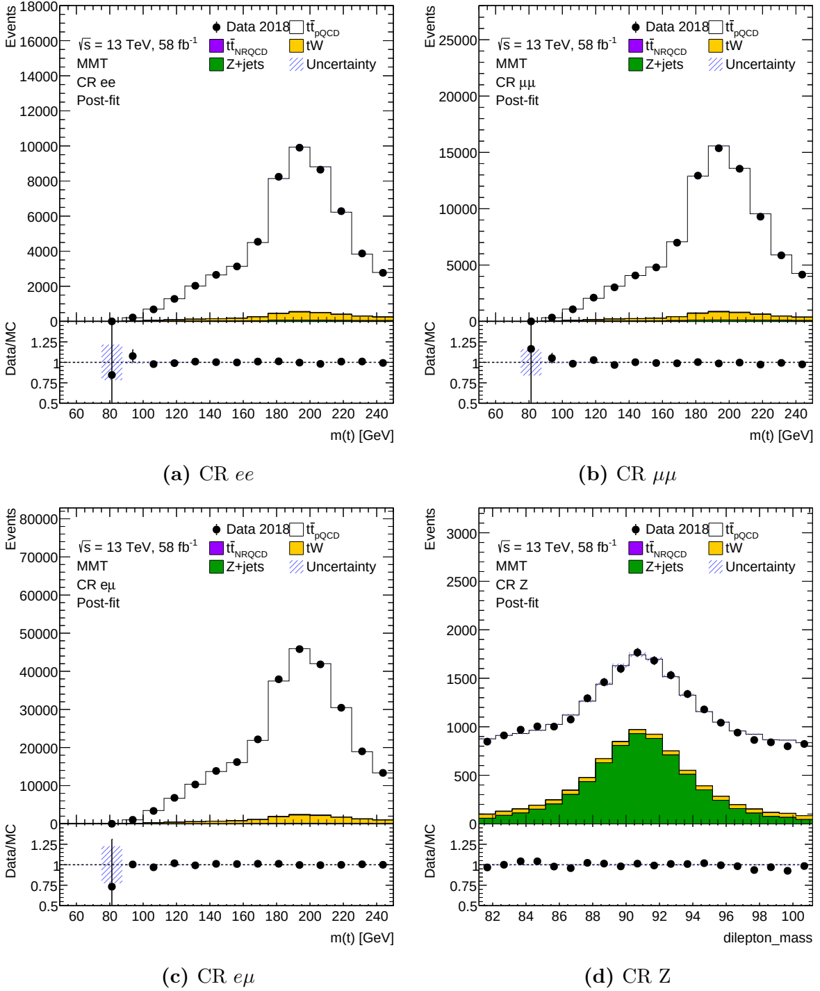
Figure A.28.: Plots showing the comparison between data and simulation of top-quark pair production and its leading backgrounds. The different control regions used in the fits are shown as stacked histograms of the different distributions, where the normalisations for t\bar{t}_{pQCD} and Z+jets are extracted from the fit as summarised in eq. (8.2). Note that the reconstruction of the t\bar{t} -system is performed using \nu -Weighter.
