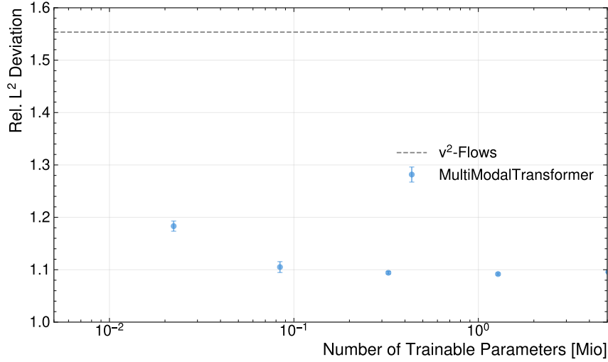
Figure 6.8.: Relative L^2 deviation of the predicted neutrino momenta compared to the true values as a function of the number of trainable parameters for the MMT architecture with nu2-Flows plotted for comparison.
