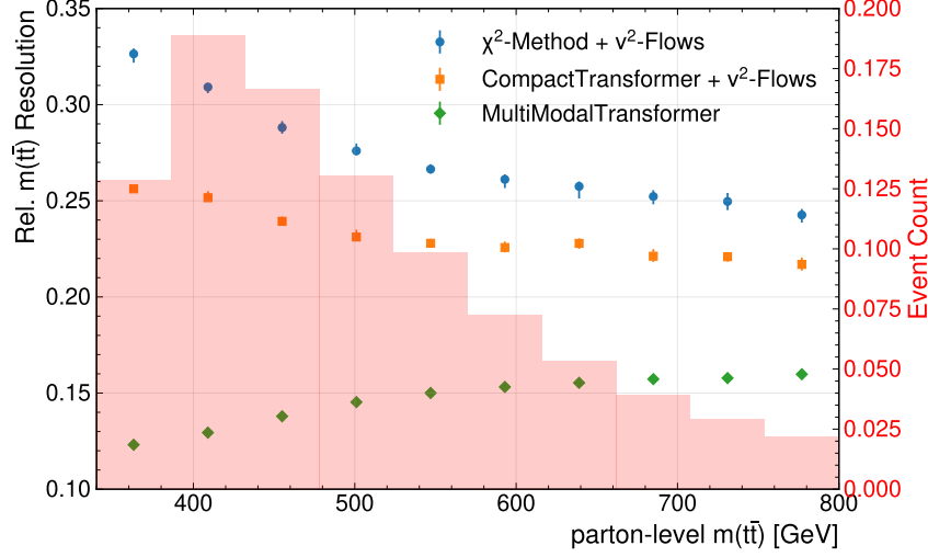
Figure 7.12.: Relative Resolution of m(t\bar{t})
