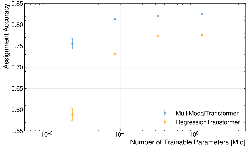
Figure A.9.: Assignment accuracy for the MultiModalTransformer and the RegressionTransformer as a function of the number of trainable parameters.
