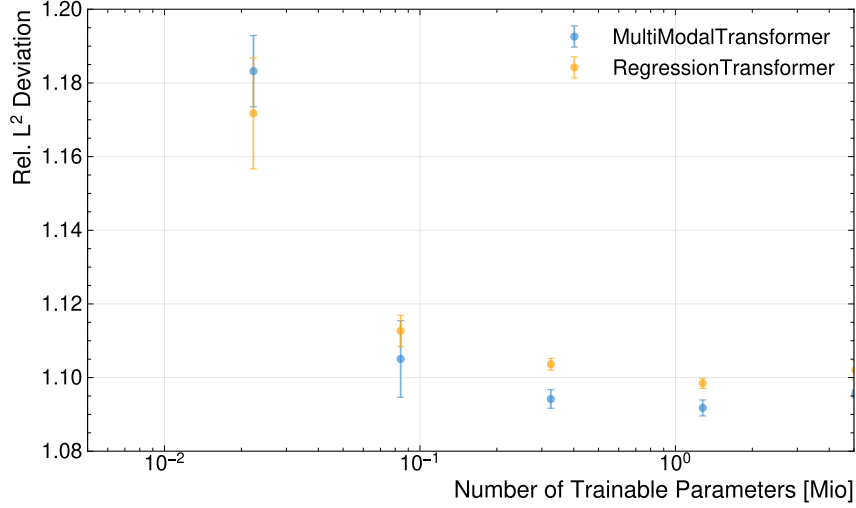
Figure 6.12.: Relative L^2 deviation of the predicted neutrino momenta compared to RegressionTransformer, which features the same architecture trained only for the neutrino regression task, as a function of the number of trainable parameters.
