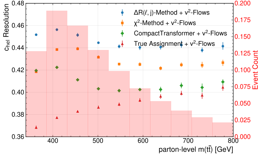
Figure 7.8.: Resolution of c_{hel}
