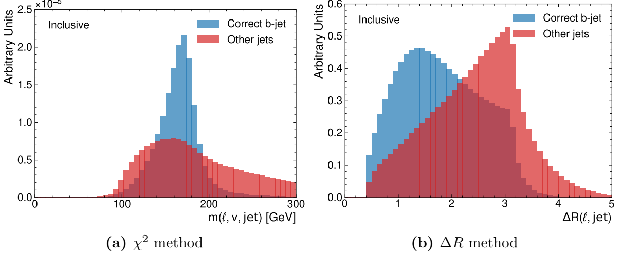
Figure 5.1.: Distributions for pairing up correct and incorrect jet-lepton pairs for the reconstructed invariant mass of the top quark (a) used for the \chi^2 method and the \Delta R between the jet and lepton (b) used for the \Delta R method. The distributions are normalised to unit area. Note that the reconstructed invariant mass for the \chi^2 method includes the neutrino prediction from \nu^2 -Flows.
