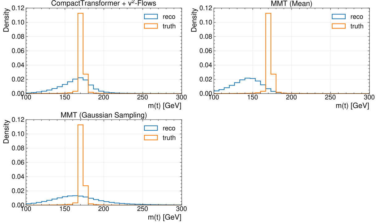
Figure A.24.: Comparison of m(t) distributions at reco- and parton-level for the different regression settings of the MultiModalTransformer trained with the Gaussian-loss.
