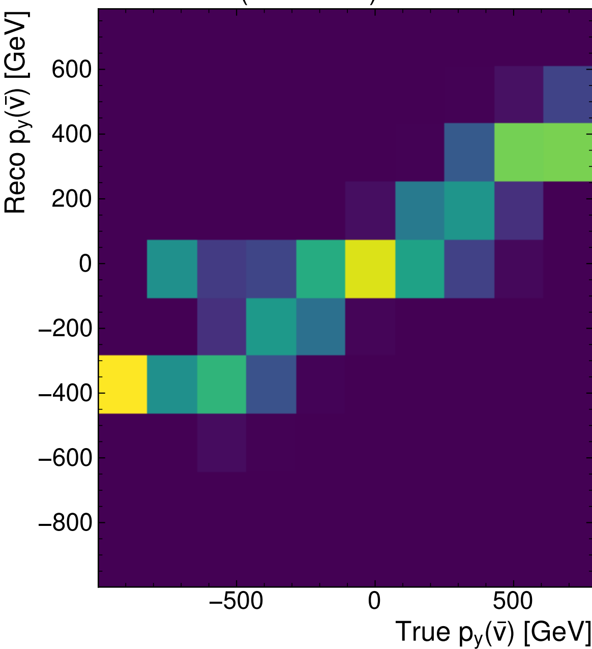
CPT (Threshold) + v^2 -Flows
