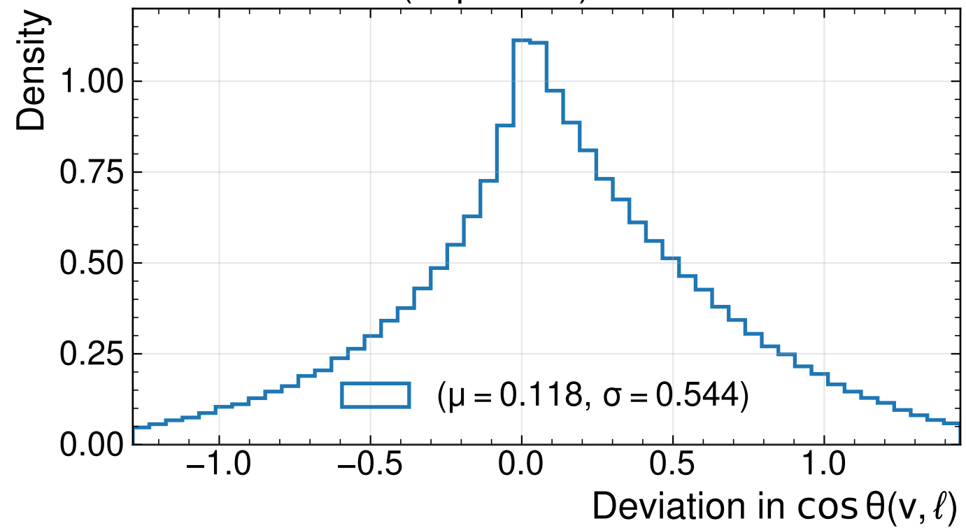
CPT (Toponium) + v^2 -Flows
