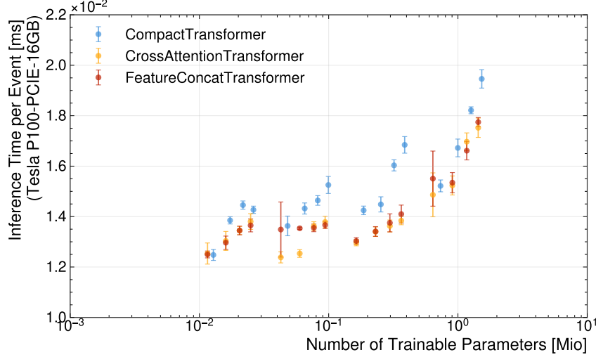
Figure 6.6.: Inference Time of all architectures as a function of the number of trainable parameters. Each point represents the average inference time over 5 runs with different random seeds and k-folded training/validation data. The error bars indicate the standard deviation across the runs. Note, that the scaling of the x-axis is logarithmic, which allows for a better visualisation of the differences in performance across different model sizes.
