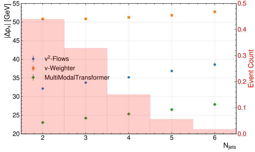
Figure A.15.: Mean absolute error of the neutrinos' p_x component binned in number jets.
