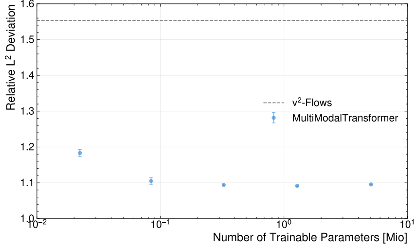
Figure 6.9.: Relative L^2 deviation of the predicted neutrino momenta compared to the true values as a function of the number of trainable parameters for the MultiModalTransformer (MMT) architecture.
