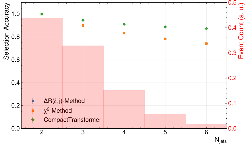
Figure A.12.: Selection accuracy as a function of the number of jets in the event for different reconstruction methods.
