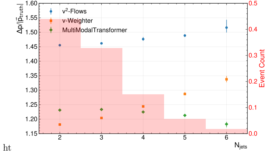
Figure 7.5.: Relative L^2 distance of the neutrino vectors binned with respect to the number of jets. The background histogram shows the distribution of events as a function of the number of jets. The uncertainties represent the statistical variations in the evaluation dataset.
