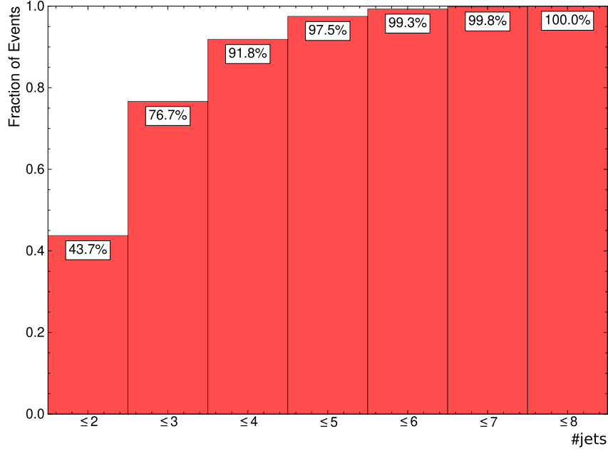
Figure 6.4.: Cumulative histogram of jet numbers per events.
