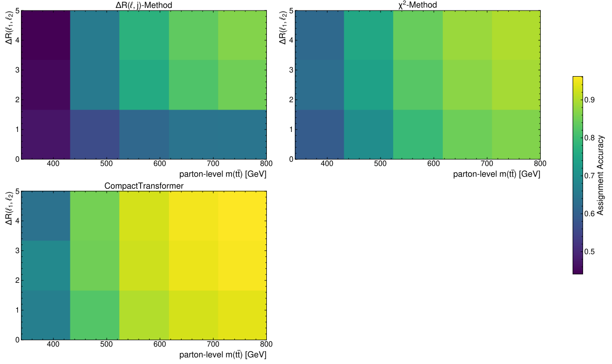
Figure A.13.: Assignment accuracy binned with respect to parton-level m(t\bar{t}) and \Delta R(\ell_1, \ell_2) .
