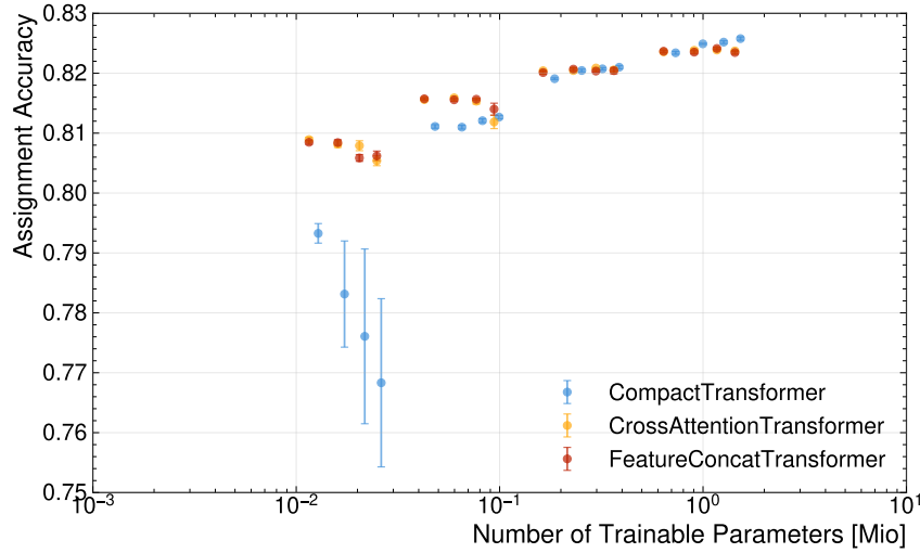
Figure 6.5.: Assignment Accuracy of all architectures as a function of the number of trainable parameters. Each point represents the average accuracy over 5 runs with different random seeds and k-folded training/validation data. The error bars indicate the standard deviation across the runs. Note, that the scaling of the x-axis is logarithmic, which allows for a better visualisation of the differences in performance across different model sizes.
