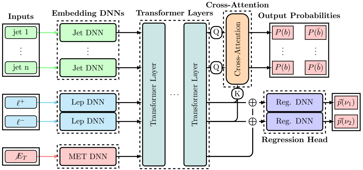
Figure 6.8.: This schematic visualises the general structure of the CompactTransformer architecture equipped with an additional head for neutrino regression. Note, that \oplus represents a concatenation of the corresponding features. This architecture is called MultiModalTransformer (MMT).
