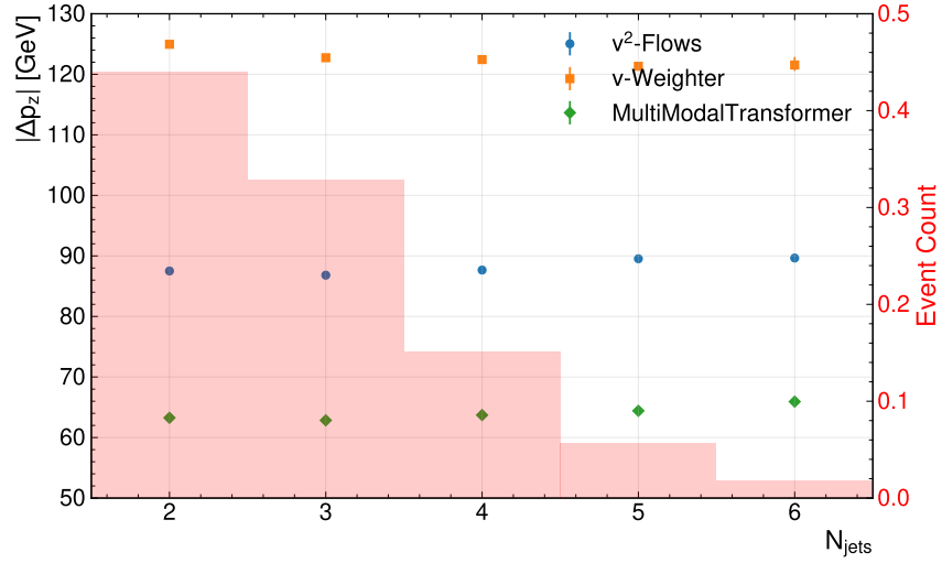
Figure A.16.: Mean absolute error of the neutrinos' p_z component binned in number jets.
