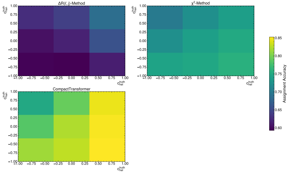
Figure A.14.: Assignment accuracy binned with respect to parton-level c_{\text{hel}} and c_{\text{chan}} .
