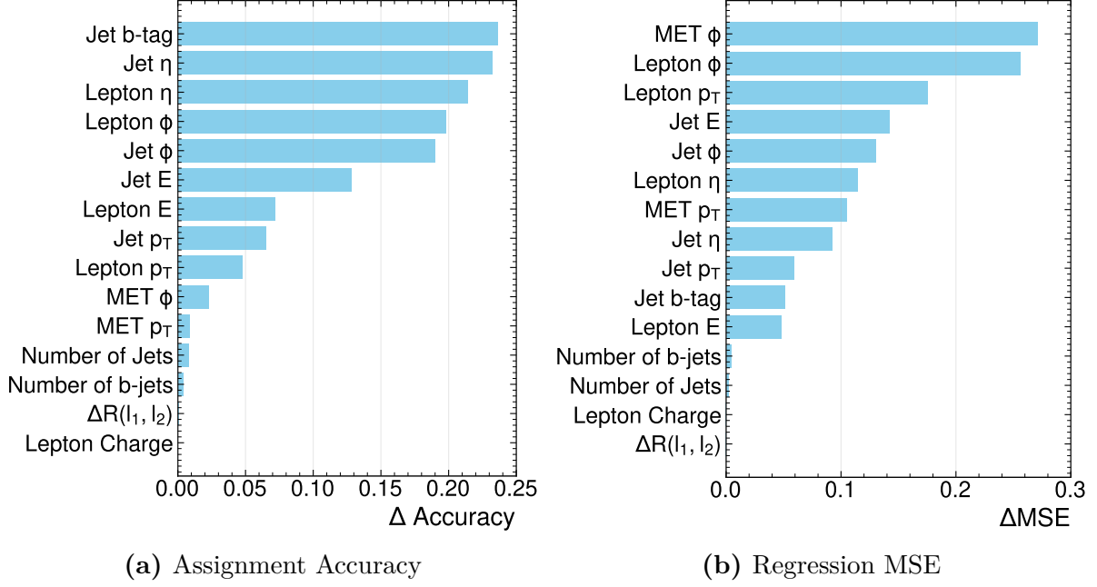
Figure 6.10.: The Plots (a) and (b) show the difference in assignment accuracy and regression MSE, respectively, of the CPT-model when permuting the input features. For each feature, five different permutation are performed. The features are ranked in decreasing order of the observed reduction. Note, that the mean-square error is again computed as the relative deviation of the L^2 -norm as before.
