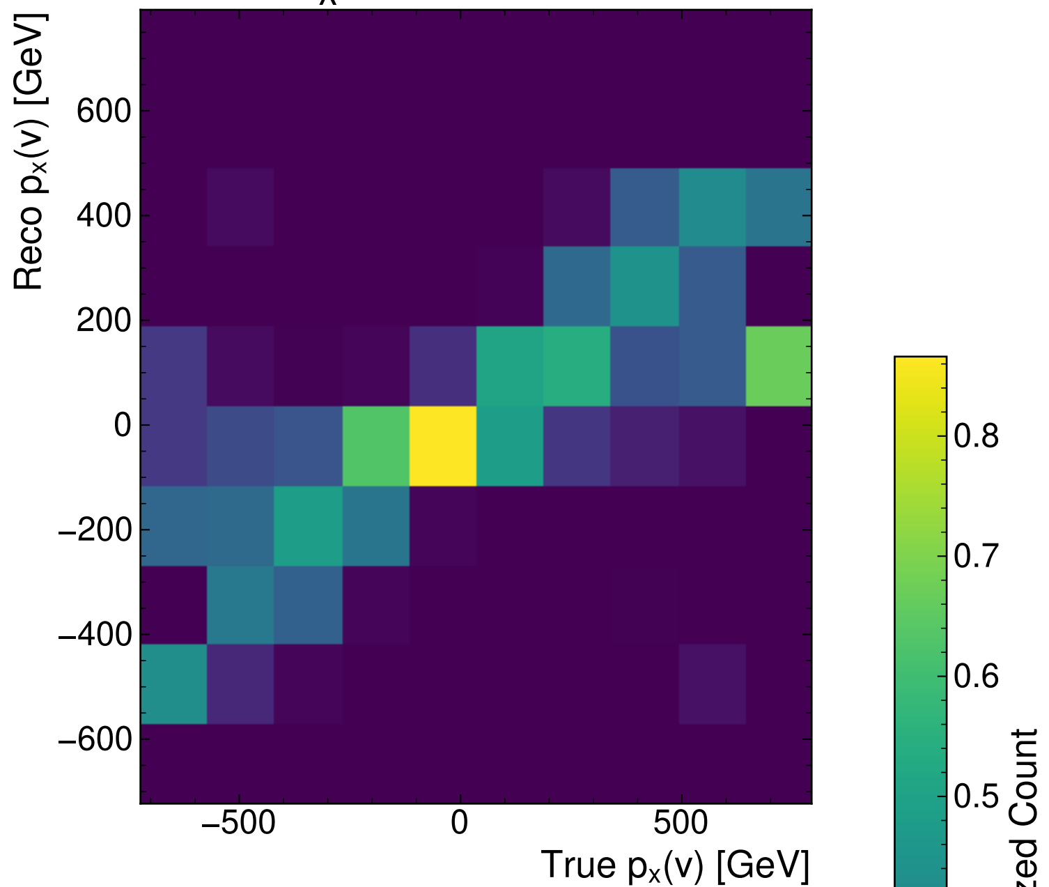
\chi^2 -Methodv 2 -Flows
