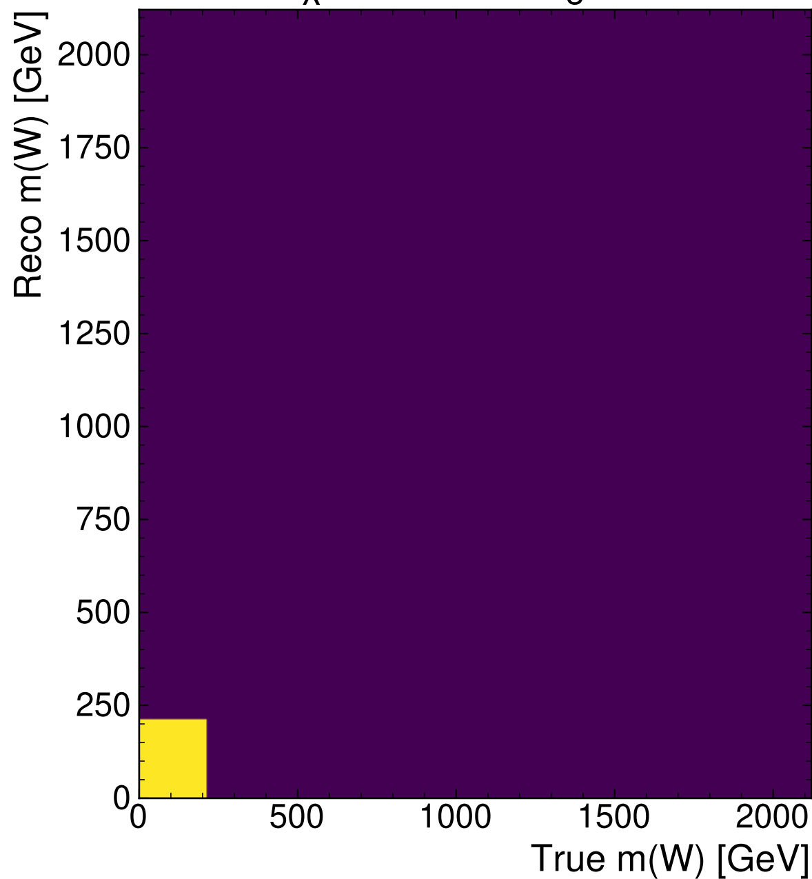
\chi^2 -Methodv-Weighter
