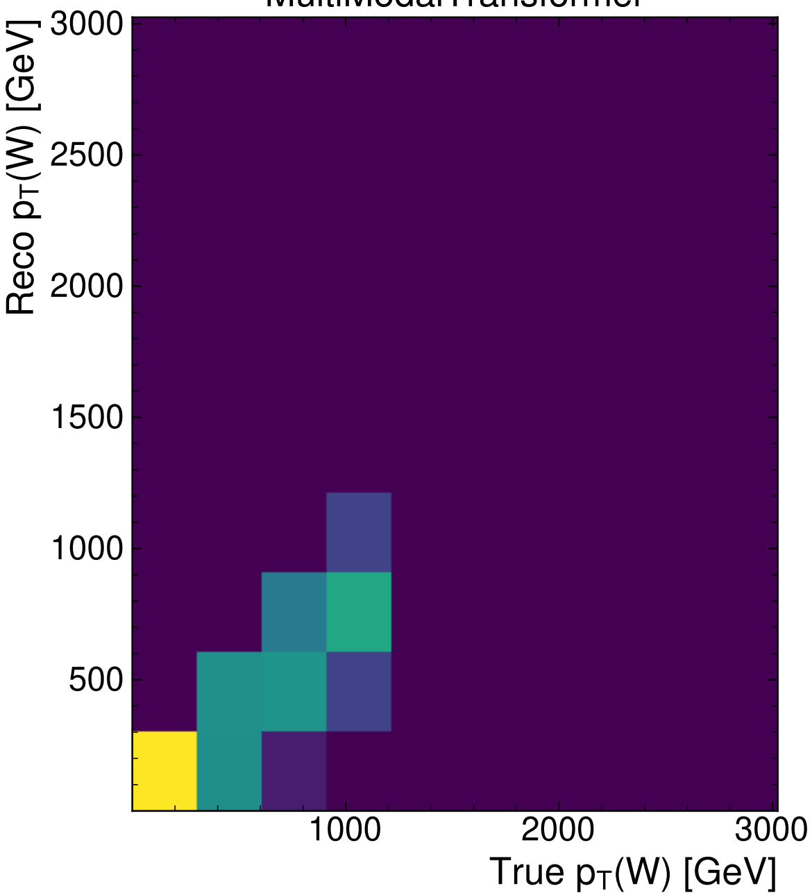
MultiModalTransformer
