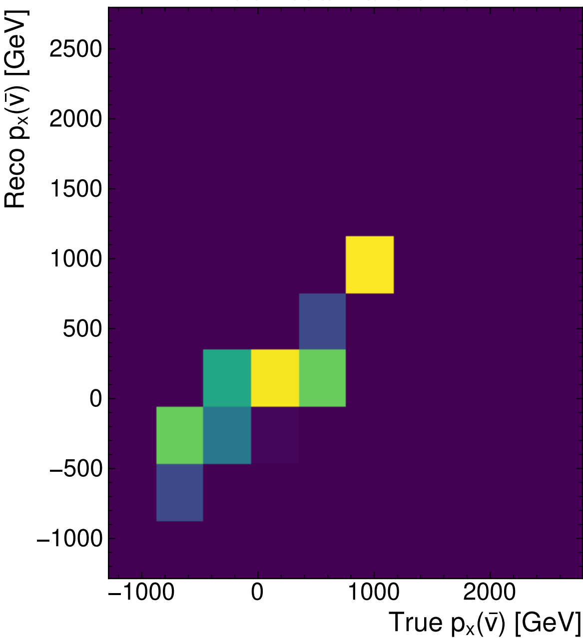
MultiModalTransformer
