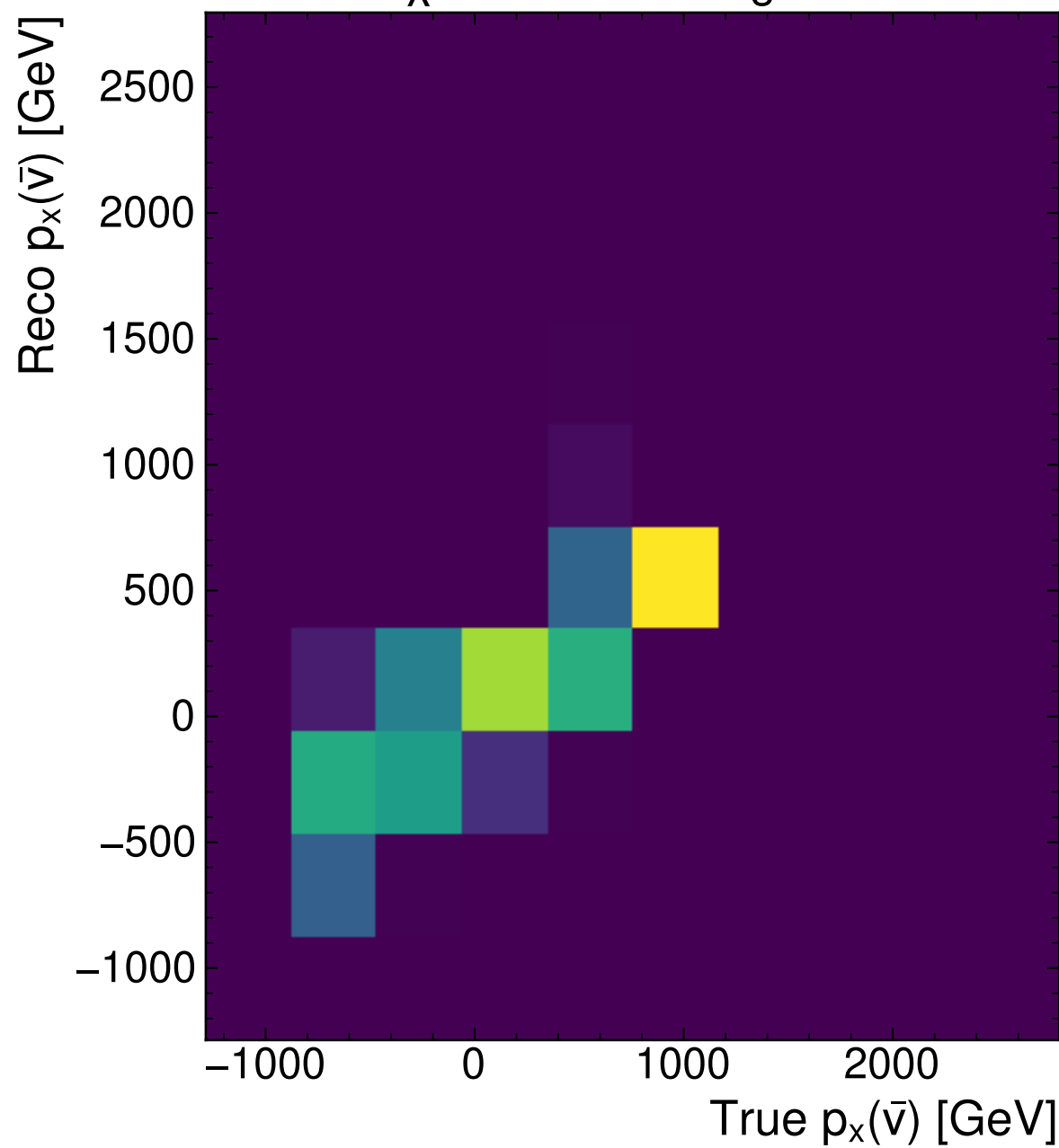
\chi^2 -Methodv-Weighter
