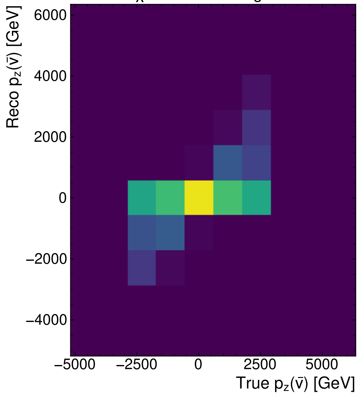
\chi^2 -Methodv-Weighter
