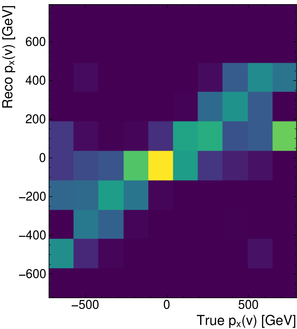
Threshold + v^2 -Flows
