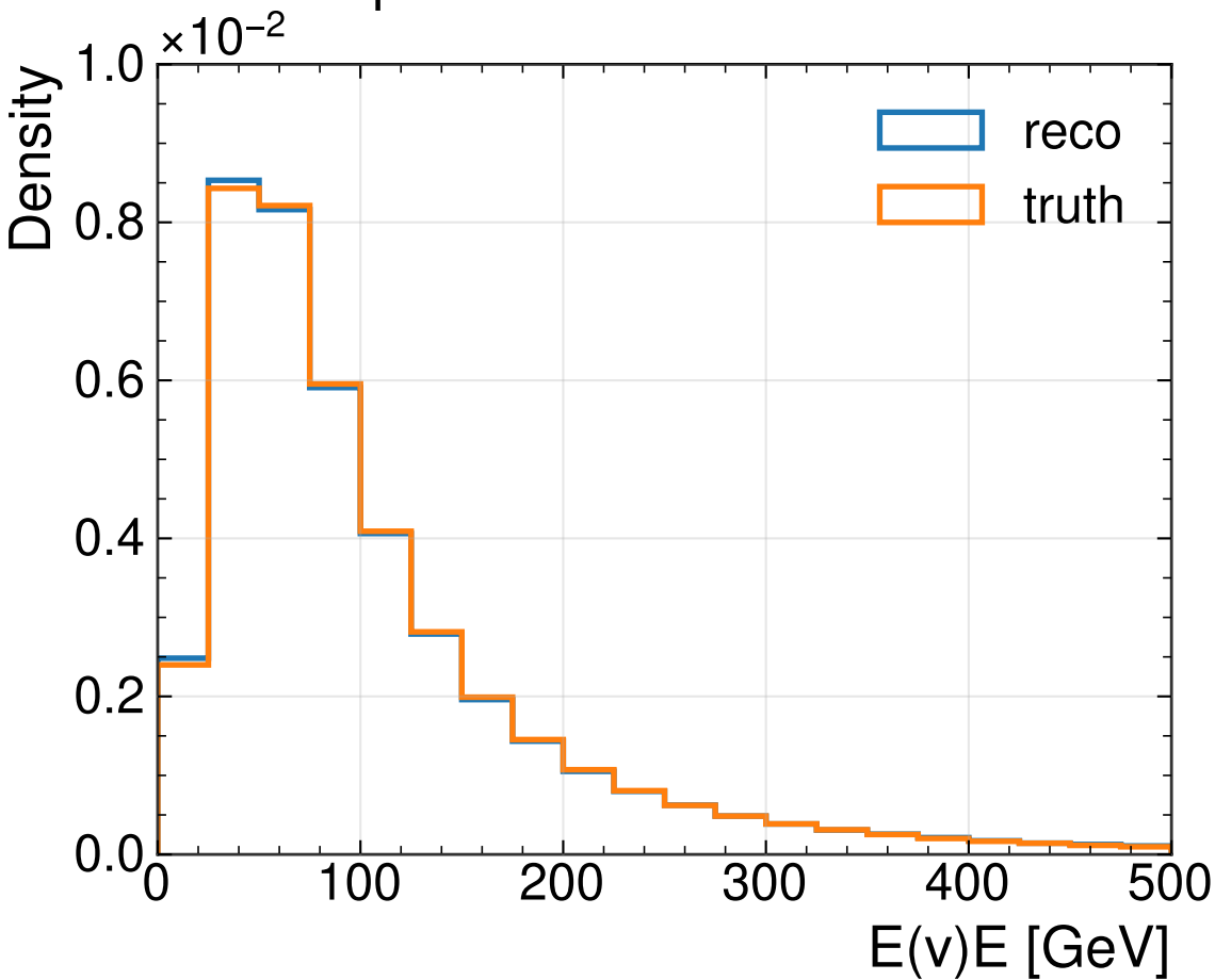
CompactTransformer + v^2 -Flows
