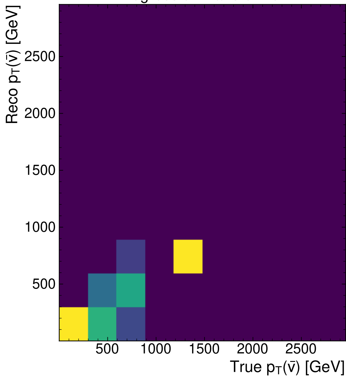
RegressionTransformer
