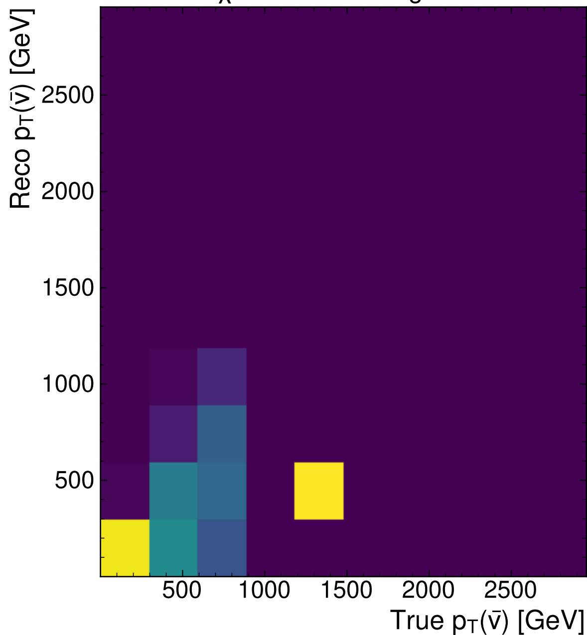
RegressionTransformer
