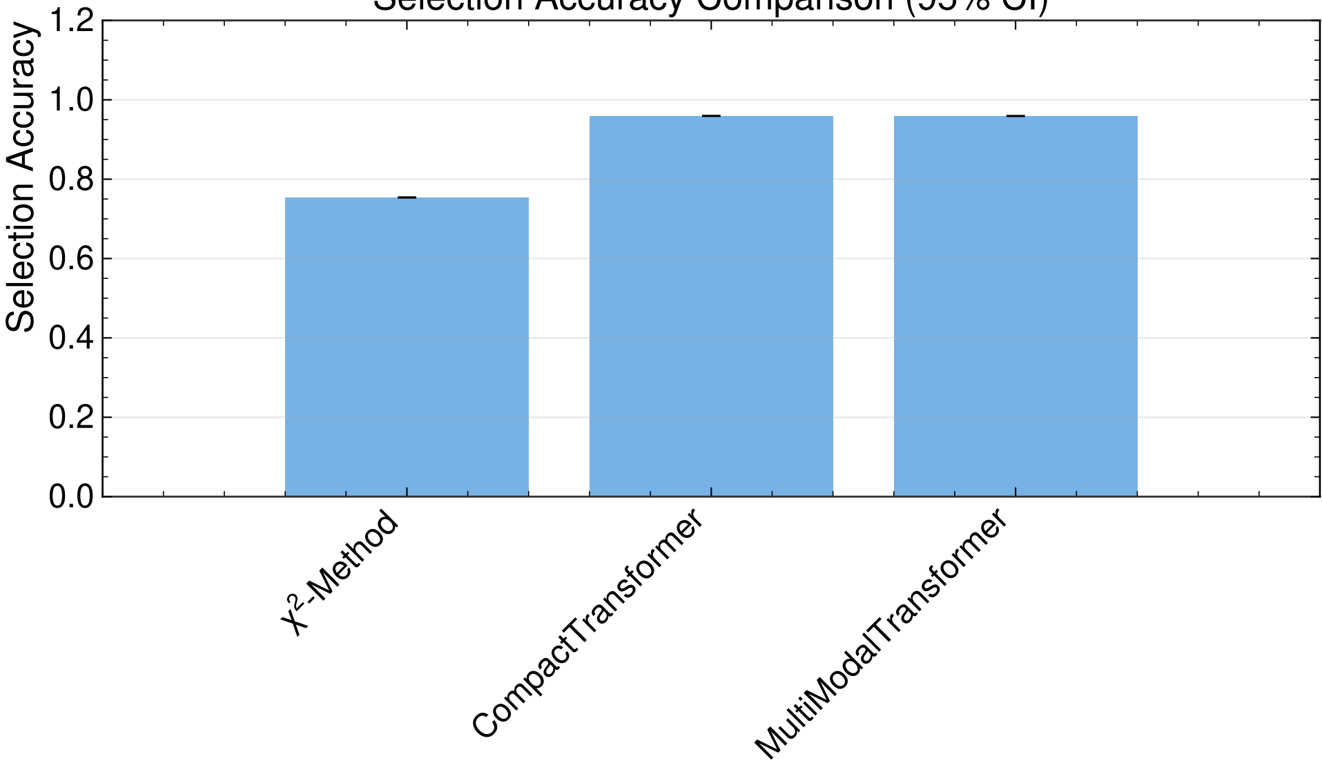
Selection Accuracy Comparison (95% CI)
