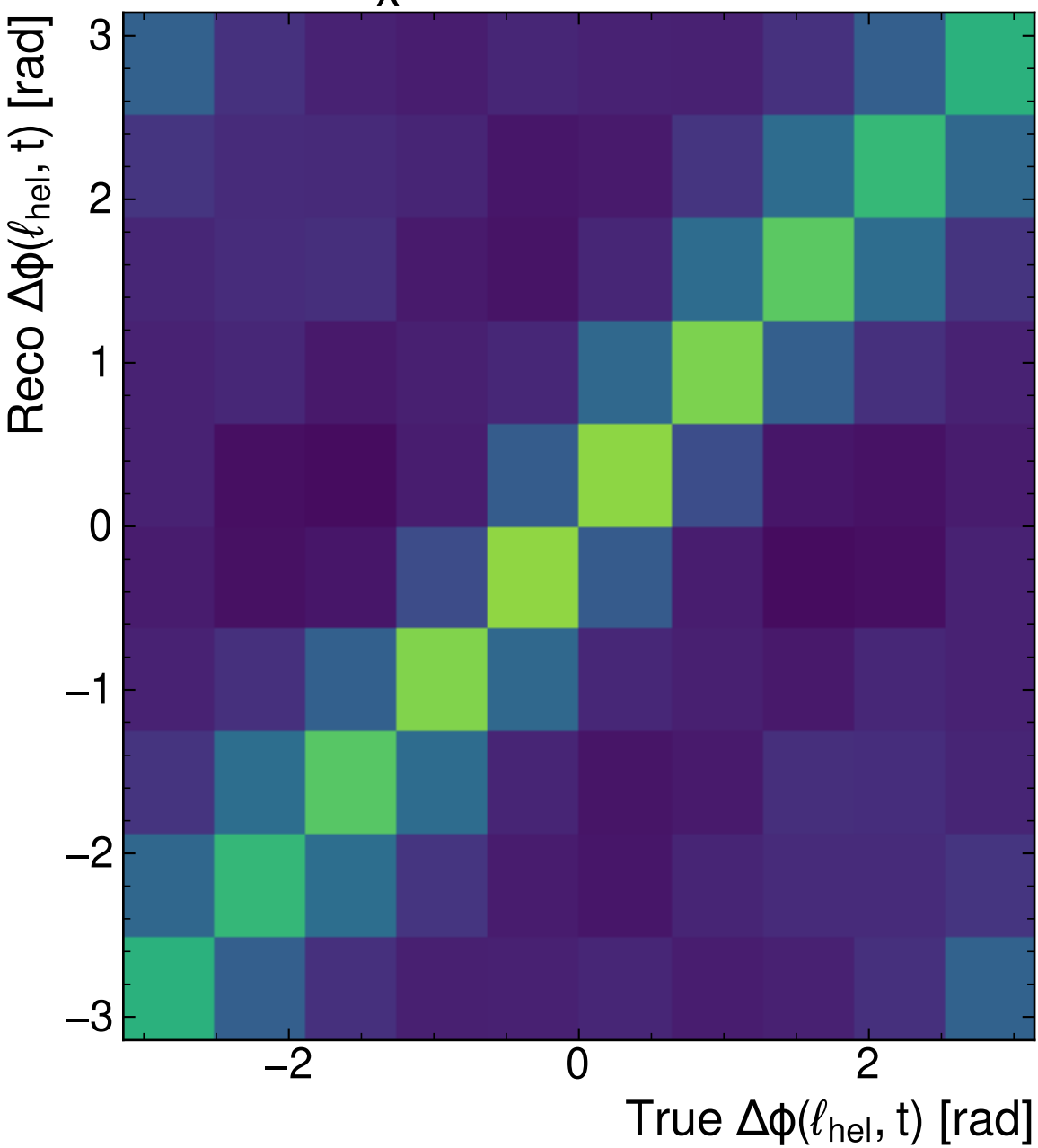
MultiModalTransformer
