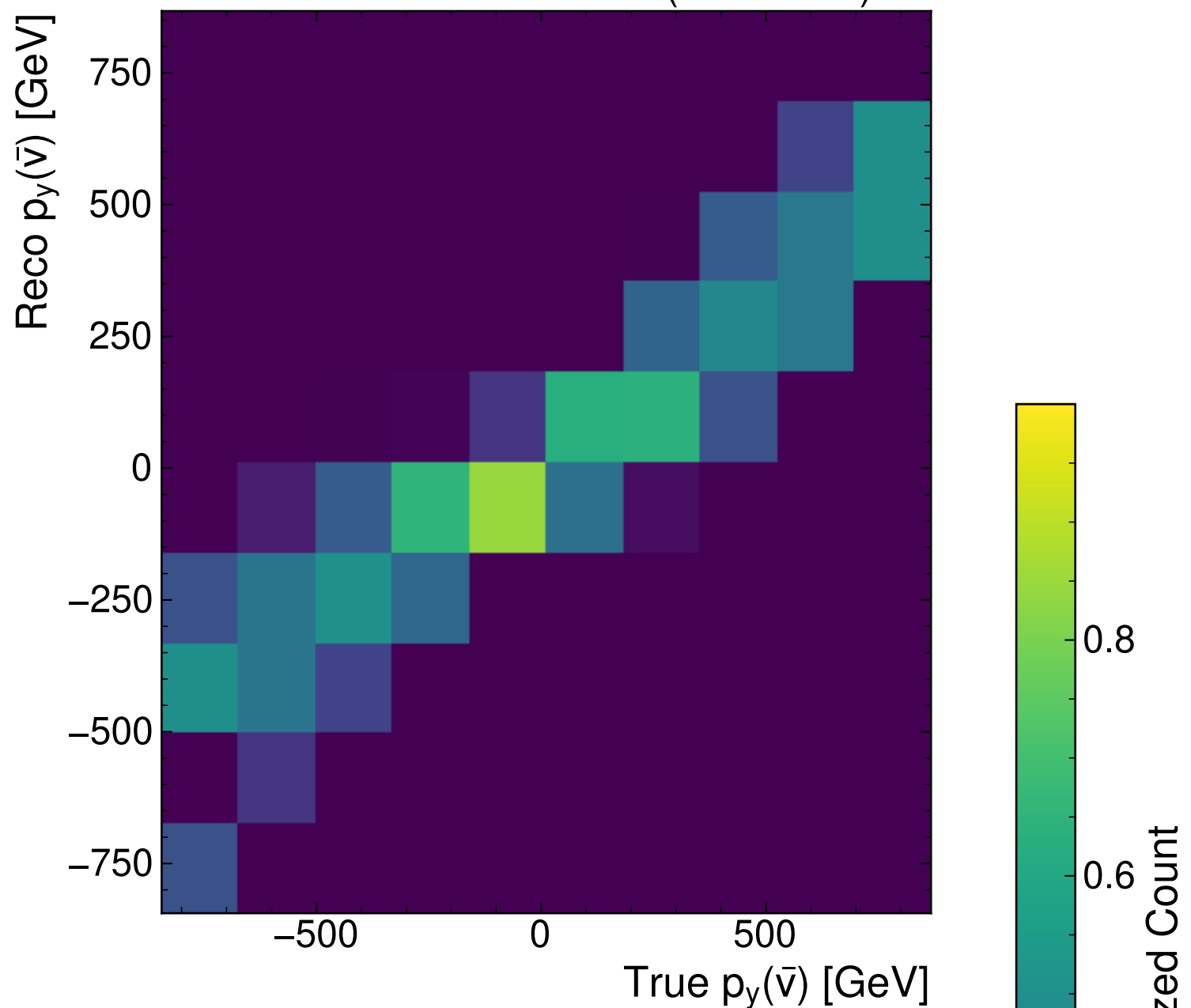
MultiModelTransformer (Magnitude-Direction)
