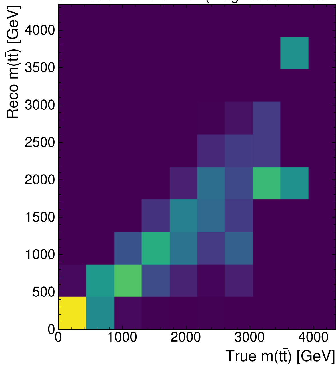
MultiModelTransformer (Magnitude-Direction)
