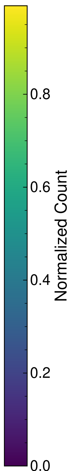
MultiModelTransformer (Magnitude-Direction)
