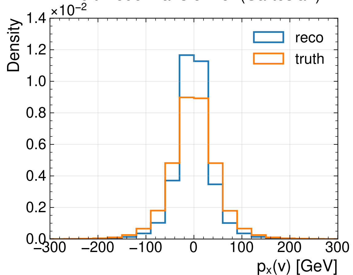
MultiModelTransformer (Magnitude-Direction)
