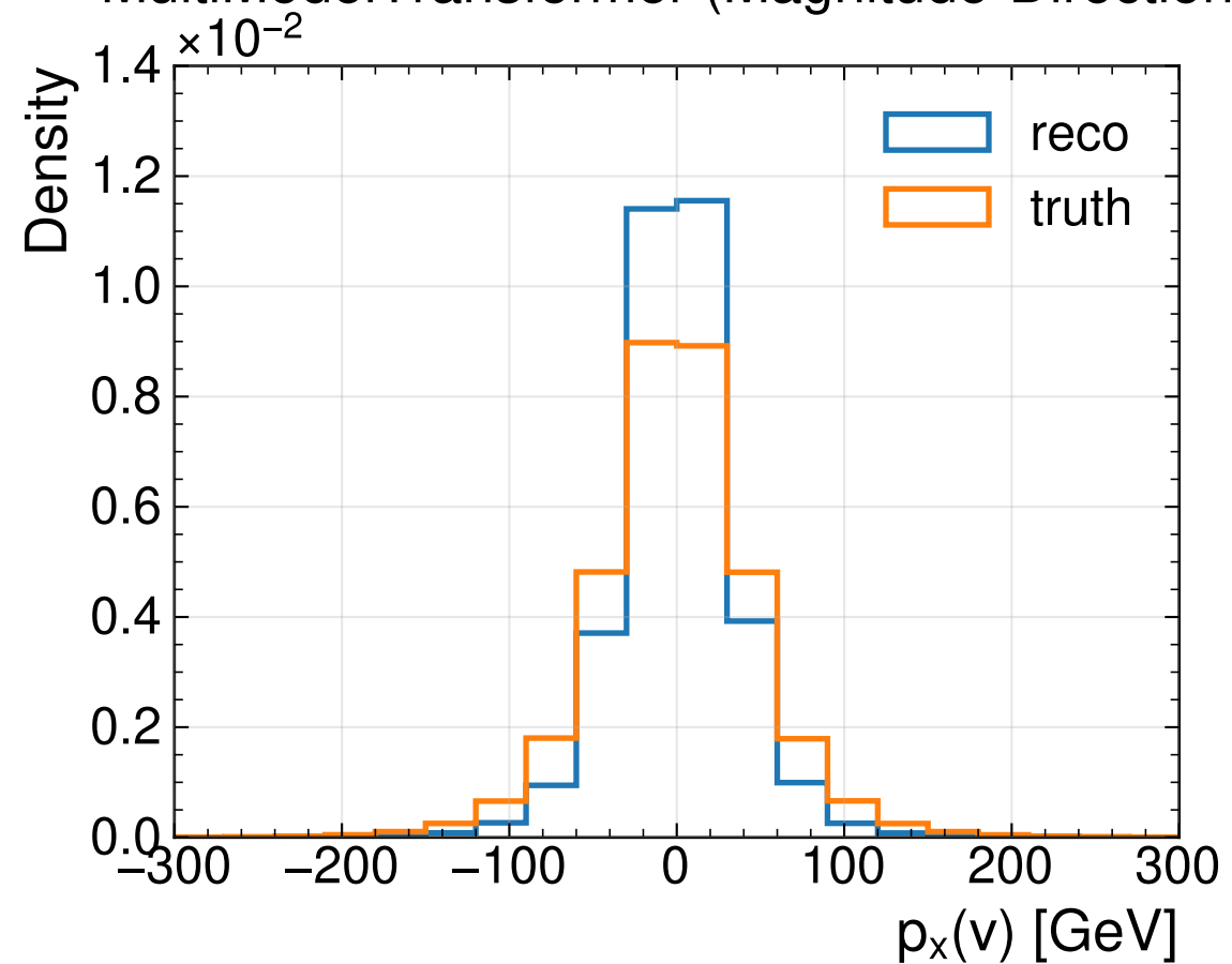
MultiModelTransformer (Magnitude-Direction)
