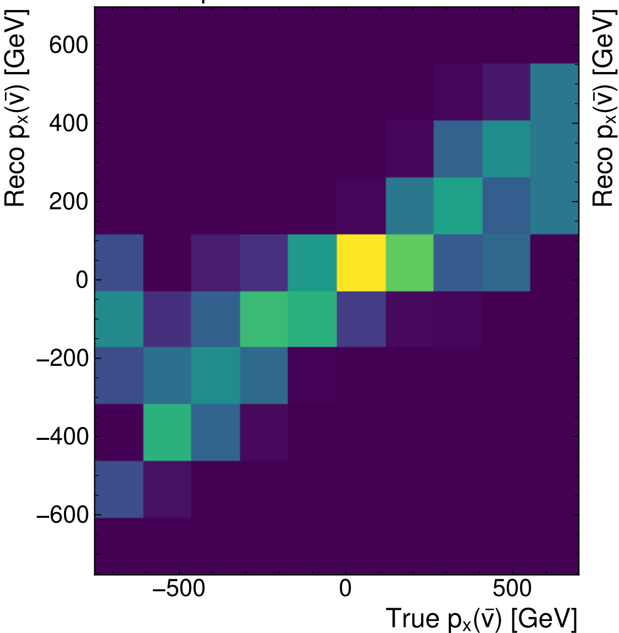
CrossAttentionTransformer + v^2 -Flows
